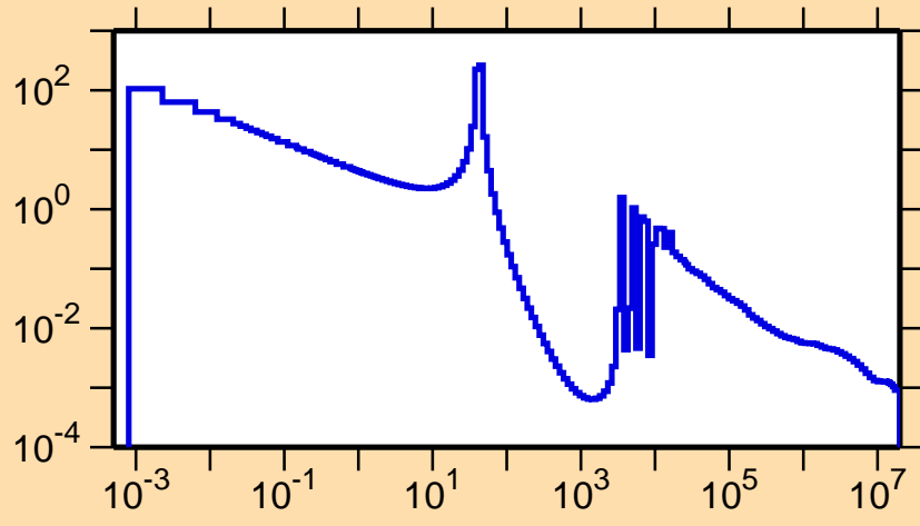
\sigma vs. E for ^{52}\text{V}(n,\gamma)
