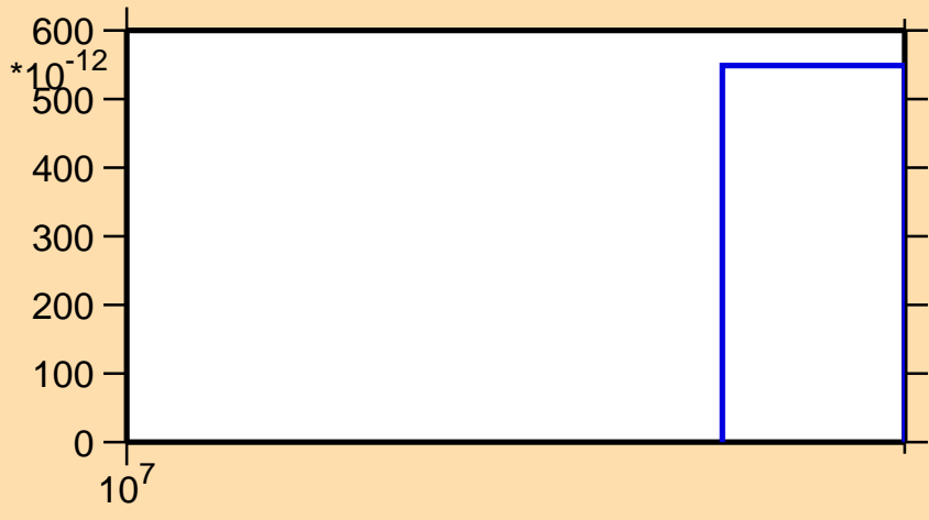
\sigma vs. E for ^{52}\text{V}(n,nt)
