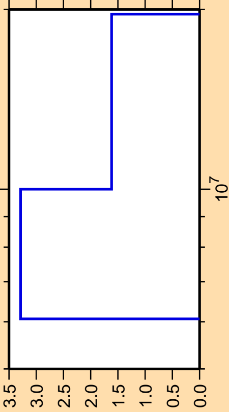
\Delta\sigma/\sigma vs. E for ^{52}\text{V}(n,2n)
