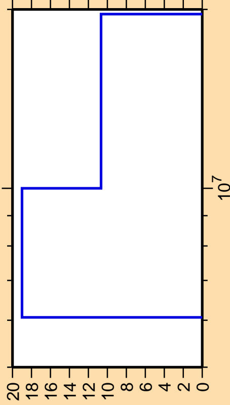
\Delta\sigma/\sigma vs. E for ^{52}\text{V}(n,n_1)
