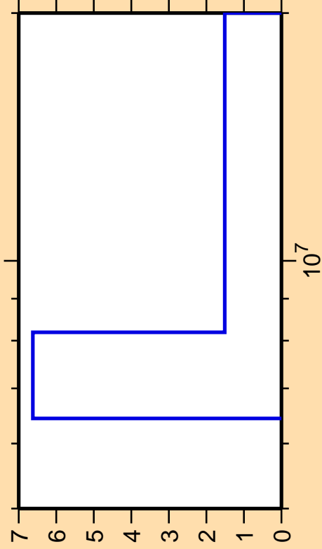
\Delta\sigma/\sigma vs. E for ^{52}\text{V}(n,2n)
