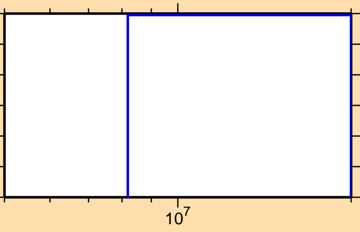
\sigma vs. E for ^{52}\text{V}(n,p\alpha)
