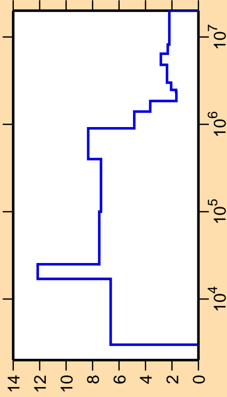
\Delta\sigma/\sigma vs. E for ^{52}\text{V}(n,\text{nonel.})
