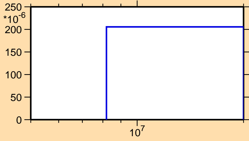
\sigma vs. E for ^{52}\text{V}(n,n\alpha)
