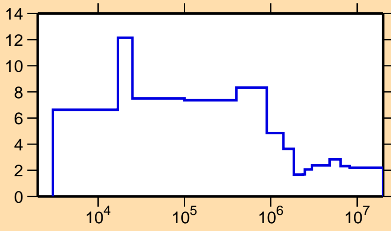
\Delta\sigma/\sigma vs. E for ^{52}\text{V}(n,\text{nonel.})
