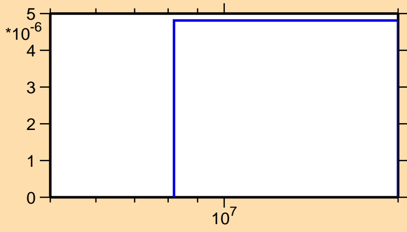
\sigma vs. E for ^{52}\text{V}(n,nd)
