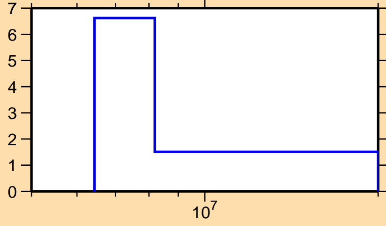
\Delta\sigma/\sigma vs. E for ^{52}\text{V}(n,2n)
