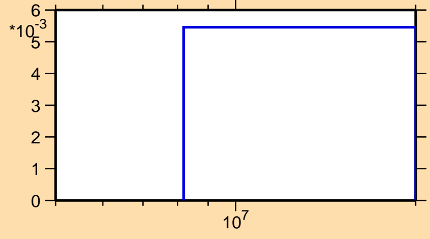
\sigma vs. E for ^{52}\text{V}(n,np)
