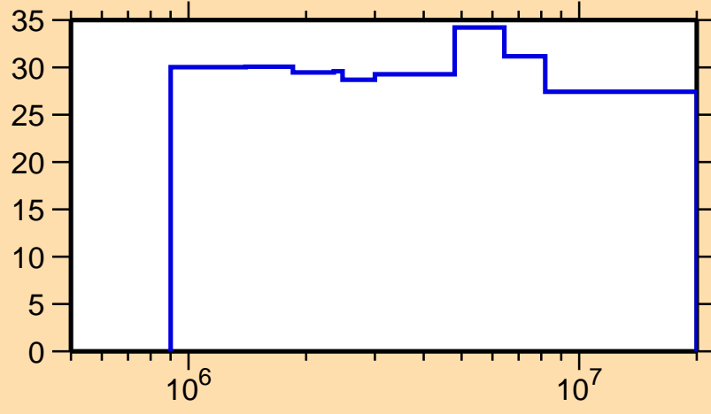
\Delta\sigma/\sigma vs. E for ^{52}\text{V}(n,\gamma)
