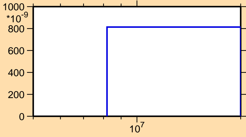
\sigma vs. E for ^{52}\text{V}(n,3n)
