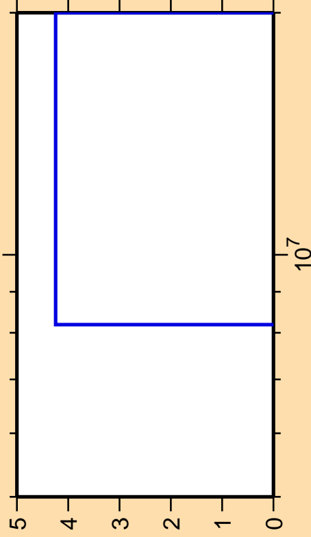
\Delta\sigma/\sigma vs. E for ^{52}\text{V}(n,nt)
