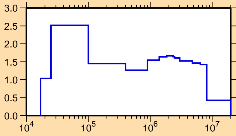
\sigma vs. E for ^{52}\text{V}(n,\text{inel.})
