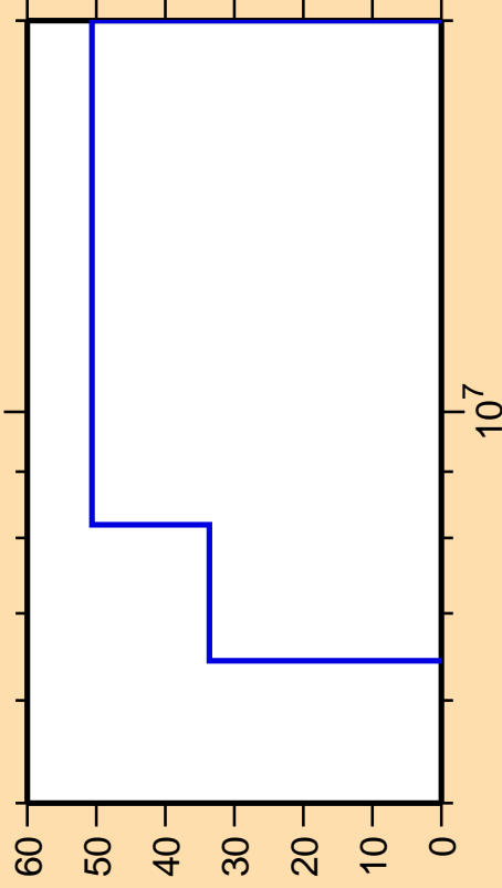
\Delta\sigma/\sigma vs. E for ^{52}\text{V}(n,t)
