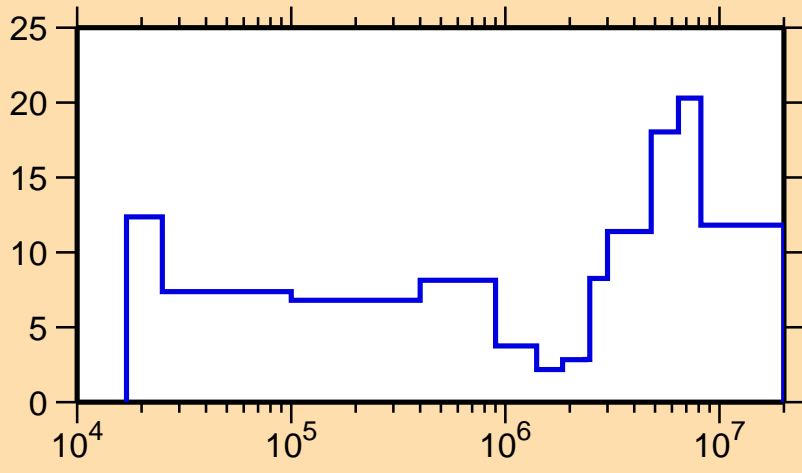
\Delta\sigma/\sigma vs. E for ^{52}\text{V}(n,n_1)
