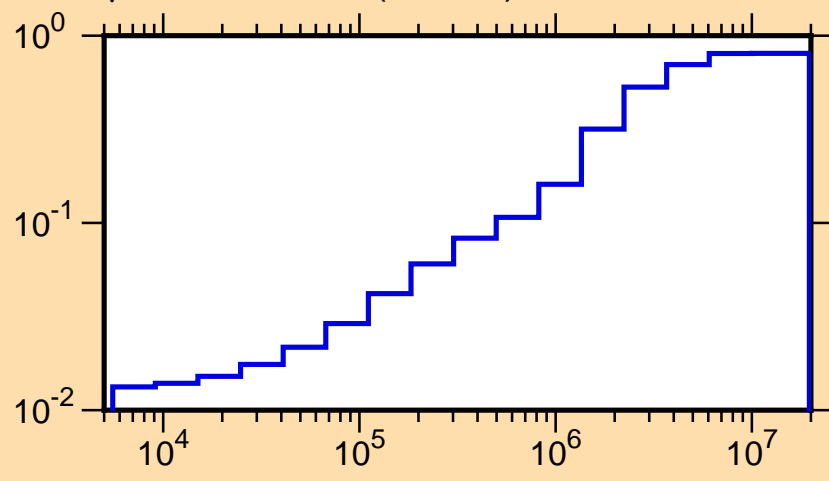
\mu vs. E for ^{53}\text{V}(\text{mt251})
