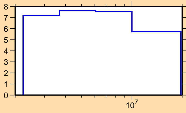
\Delta\sigma/\sigma vs. E for ^{53}\text{V}(n,\text{el.})
