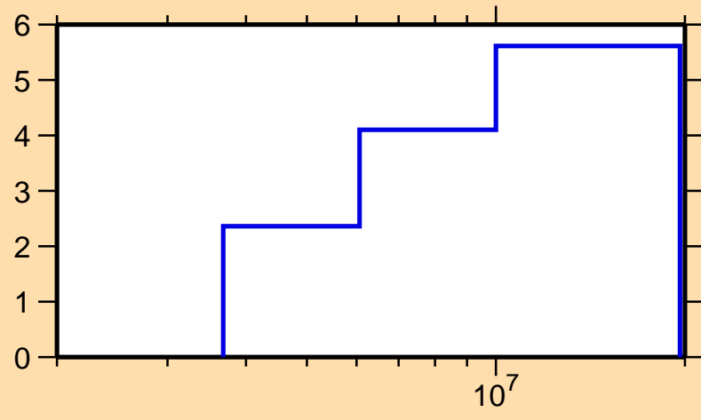
\Delta\sigma/\sigma vs. E for ^{53}\text{V}(n,tot.)
