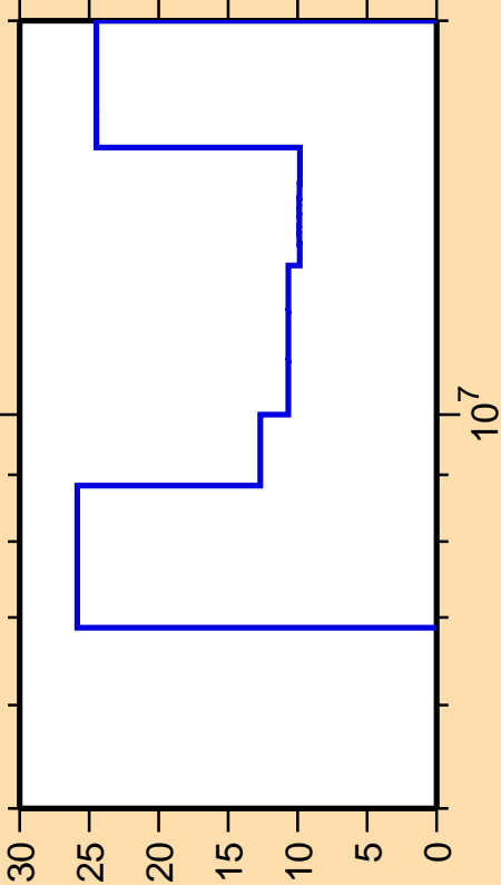
\Delta\sigma/\sigma vs. E for ^{55}\text{V}(n,2n)
