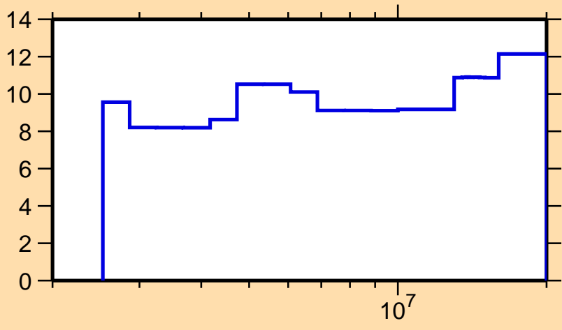
\Delta\sigma/\sigma vs. E for ^{55}\text{V}(n,n\text{onel.})
