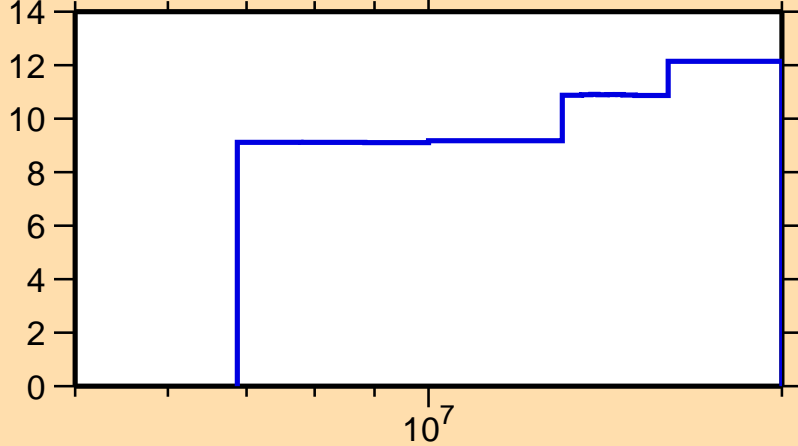
\Delta\sigma/\sigma vs. E for ^{55}\text{V}(n,\text{nonel.})
