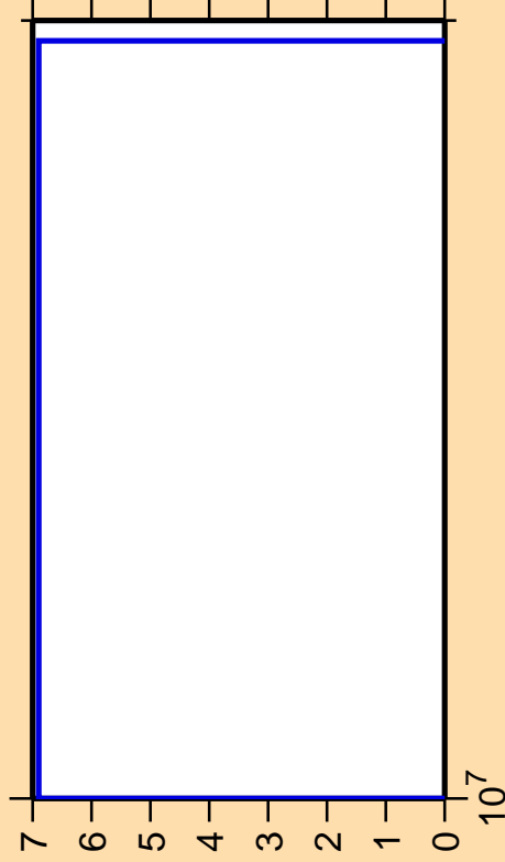
\Delta\sigma/\sigma vs. E for ^{55}\text{V}(n,2n\alpha)
