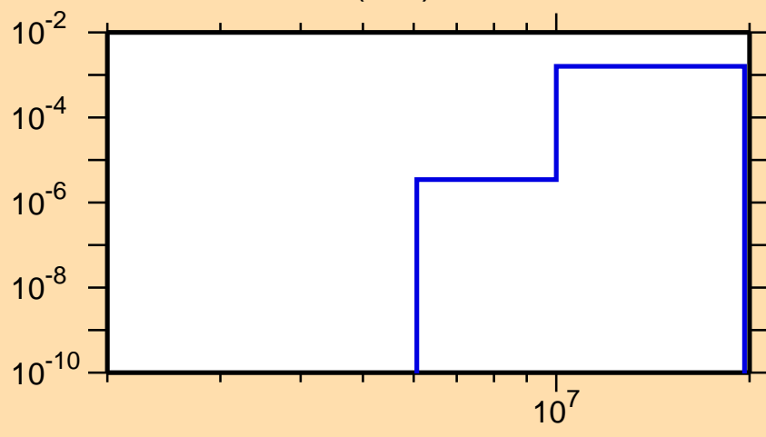
\sigma vs. E for ^{55}\text{V}(n,\alpha)
