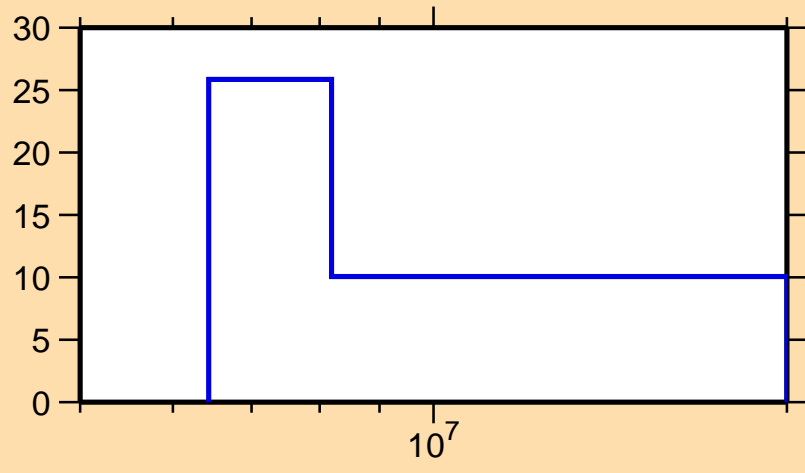
\Delta\sigma/\sigma vs. E for ^{55}\text{V}(n,2n)
