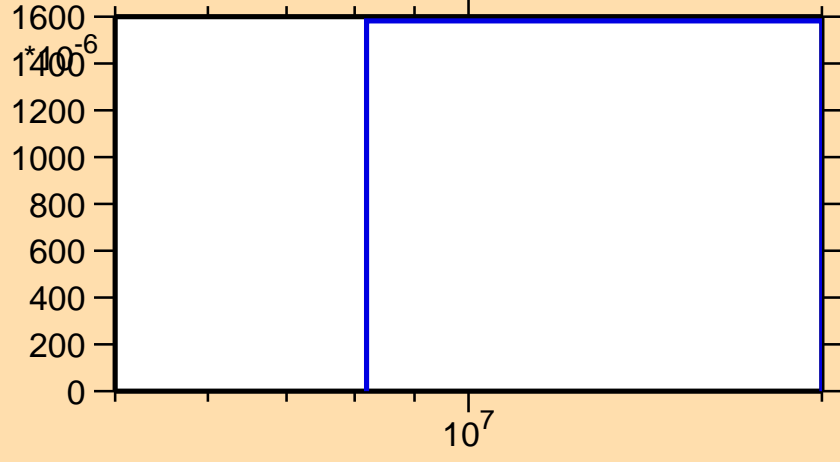
\sigma vs. E for ^{55}\text{V}(n,d)
