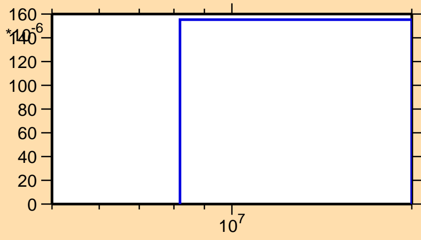
\sigma vs. E for ^{55}\text{V}(n,n\alpha)
