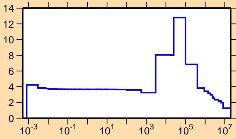
\sigma vs. E for ^{55}\text{V}(n,\text{el.})
