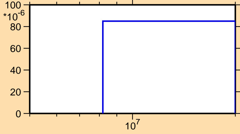
\sigma vs. E for ^{162}\text{W}(n,t)
