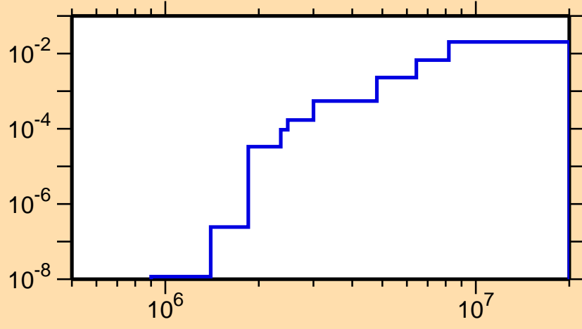
\sigma vs. E for ^{162}\text{W}(n,n\alpha)
