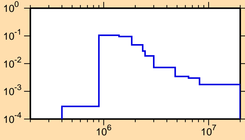
\sigma vs. E for ^{162}\text{W}(n,n_2)
