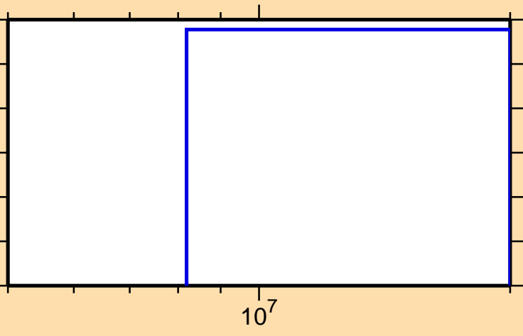
\sigma vs. E for ^{162}\text{W}(n,\text{pt})
