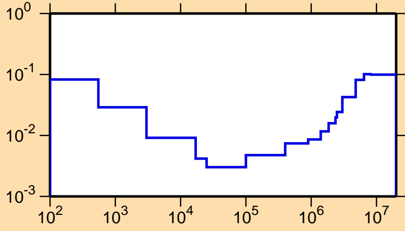
\sigma vs. E for ^{162}\text{W}(n,p\alpha)
