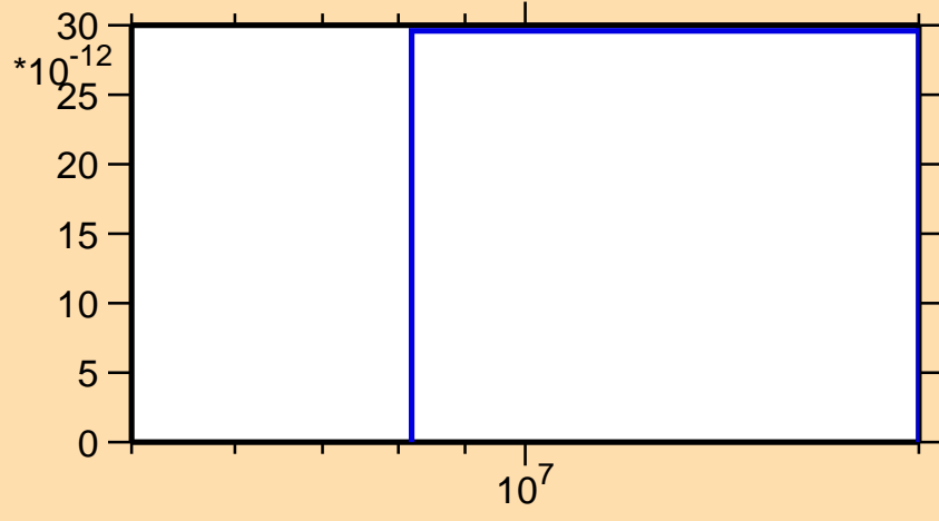
\sigma vs. E for ^{162}\text{W} (mt 34)
