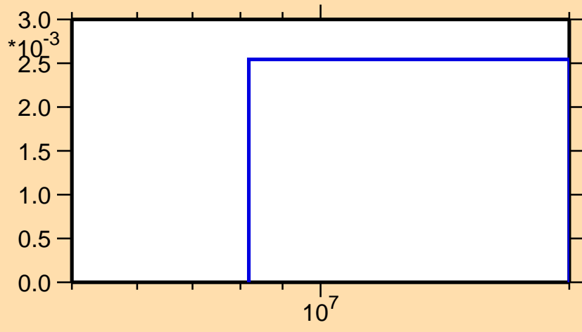
\sigma vs. E for ^{162}\text{W}(n,2n\alpha)
