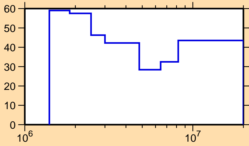
\Delta\sigma/\sigma vs. E for ^{162}\text{W}(n,ncont.)
