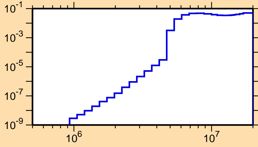
\sigma vs. E for ^{163}\text{W}(n,n\alpha)
