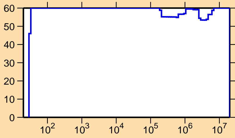
\Delta\sigma/\sigma vs. E for ^{163}\text{W}(n,p)
