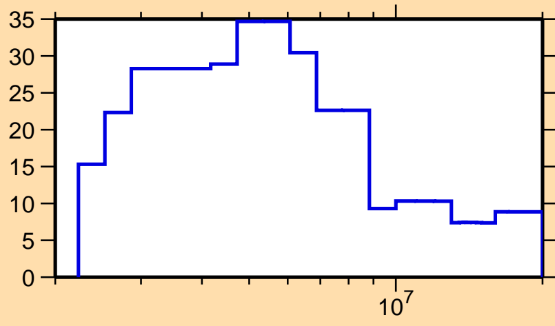
\Delta\sigma/\sigma vs. E for ^{163}\text{W}(n, el.)
