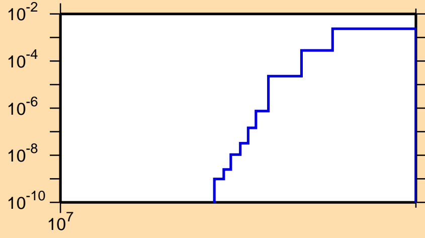
\sigma vs. E for ^{163}\text{W}(n,2np)
