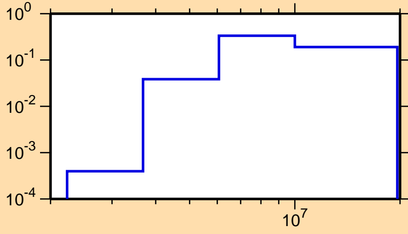
\sigma vs. E for ^{163}\text{W}(n,n\text{cont.})
