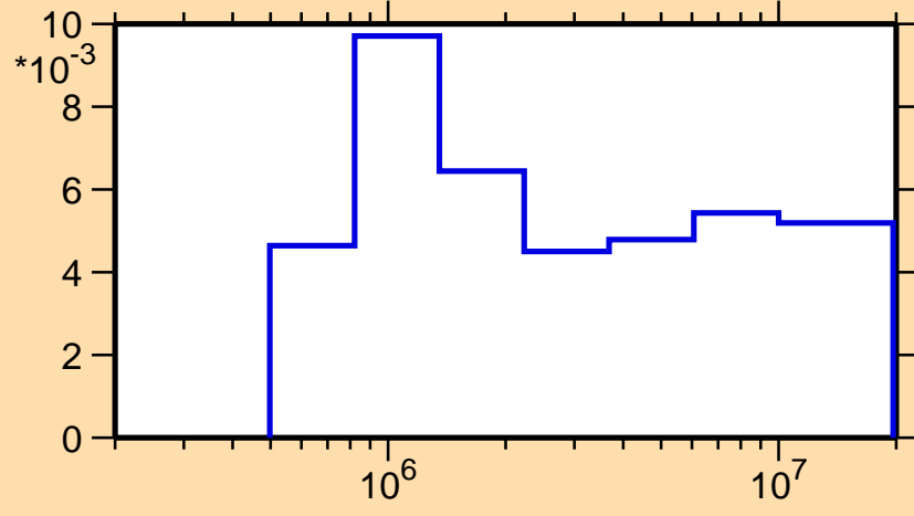
\sigma vs. E for ^{163}\text{W}(n,n_4)
