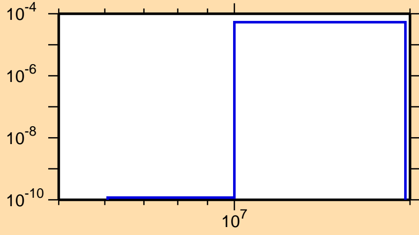
\sigma vs. E for ^{163}\text{W}(n,\text{pd})
