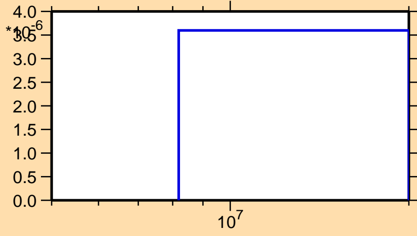
\sigma vs. E for ^{163}\text{W}(n,\text{pt})
