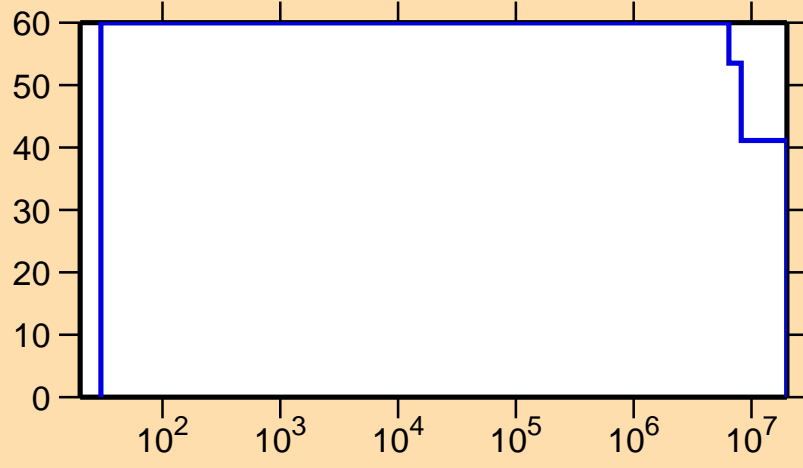
\Delta\sigma/\sigma vs. E for ^{163}\text{W}(n,\gamma)
