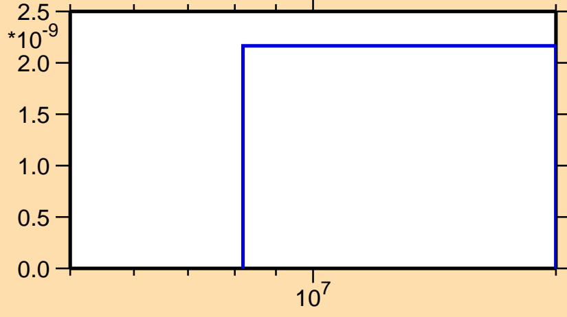
\sigma vs. E for ^{163}\text{W} (mt 34)
