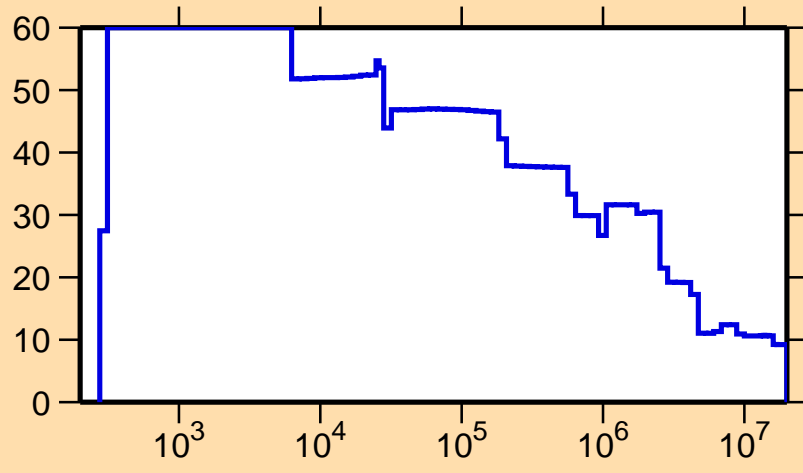
\Delta\sigma/\sigma vs. E for ^{164}\text{W}(n,\text{nonel.})
