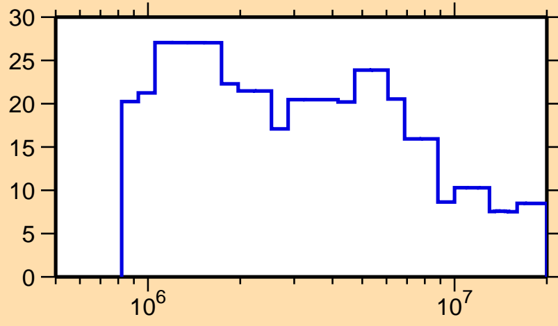
\Delta\sigma/\sigma vs. E for ^{164}\text{W}(n, el.)
