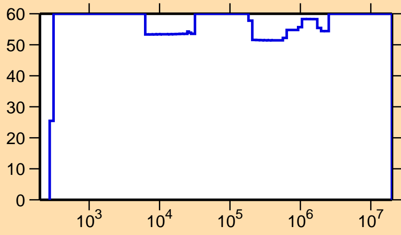
\Delta\sigma/\sigma vs. E for ^{164}\text{W}(n,\gamma)
