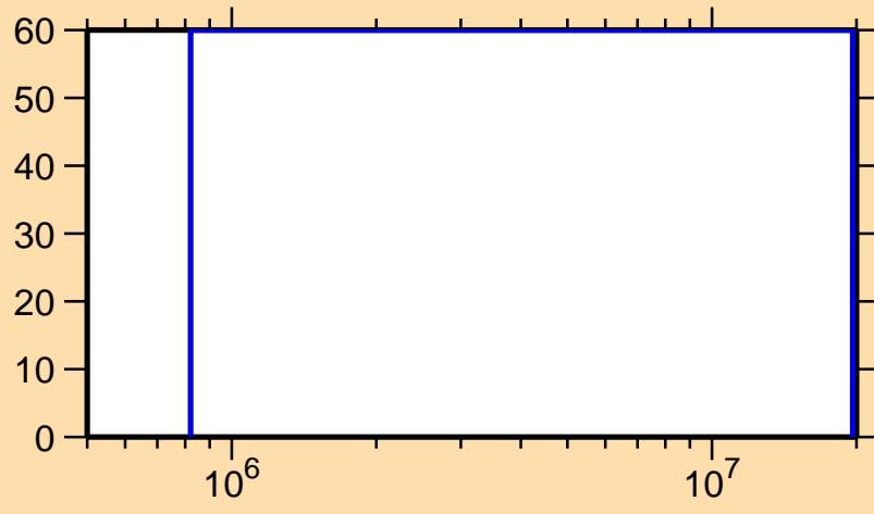
\Delta\sigma/\sigma vs. E for ^{164}\text{W}(n,ncont.)
