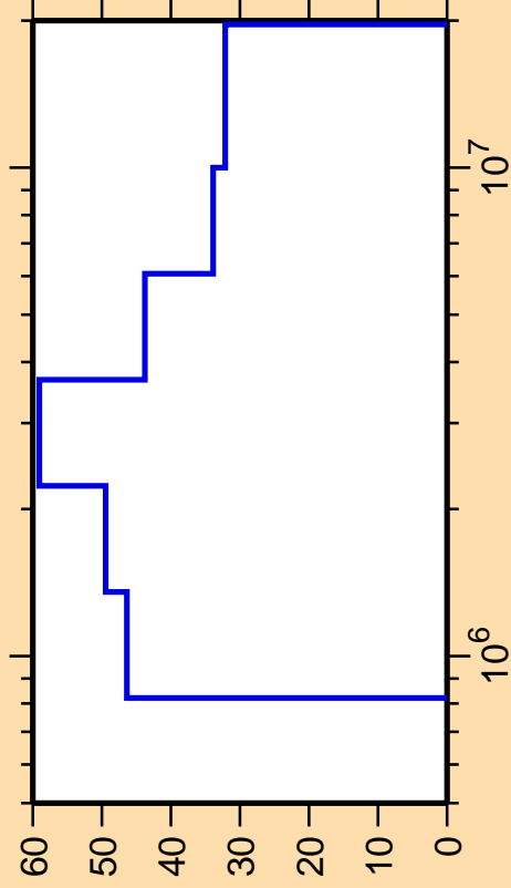
\Delta\sigma/\sigma vs. E for ^{164}\text{W}(n,n_2)
