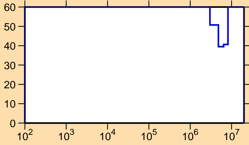
\Delta\sigma/\sigma vs. E for ^{164}\text{W}(n,p)
