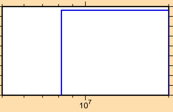
\sigma vs. E for ^{164}\text{W}(n,\text{nd})
