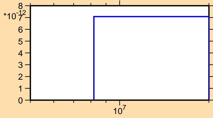
\sigma vs. E for ^{164}\text{W} (mt 34)
