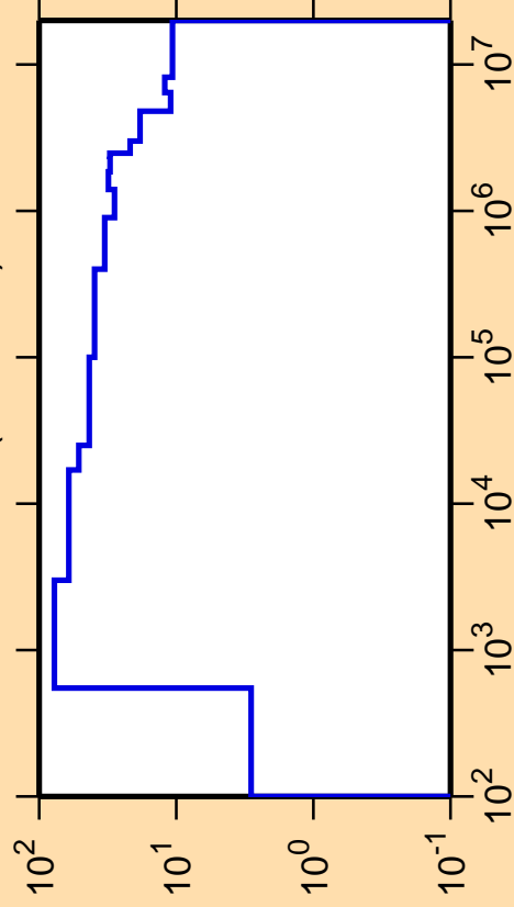
\Delta\sigma/\sigma vs. E for ^{164}\text{W}(n,\text{nonel.})
