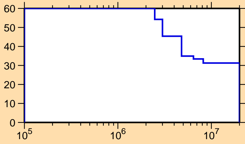
\Delta\sigma/\sigma vs. E for ^{164}\text{W}(n,n_1)
