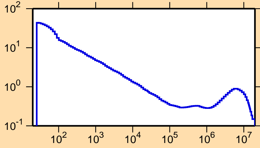
\sigma vs. E for ^{165}\text{W}(n,p)
