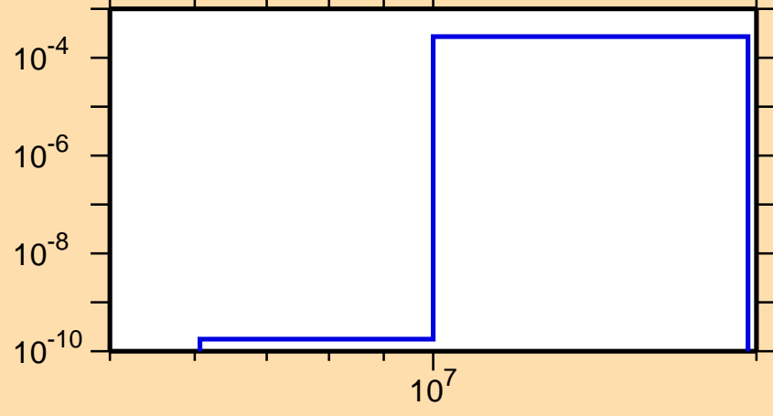
\sigma vs. E for ^{165}\text{W}(n,t)
