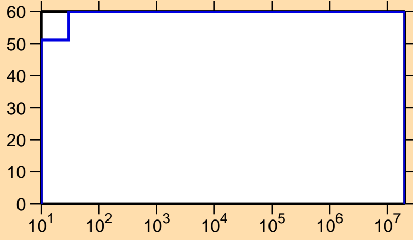
\Delta\sigma/\sigma vs. E for ^{165}\text{W}(n,\gamma)
