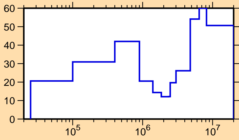
\Delta\sigma/\sigma vs. E for ^{165}\text{W}(n,\text{tot.})
