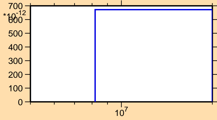
\sigma vs. E for ^{165}\text{W} (mt 34)
