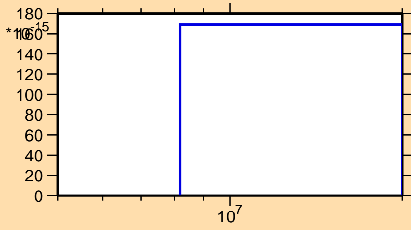
\sigma vs. E for ^{165}\text{W}(n,nt)
