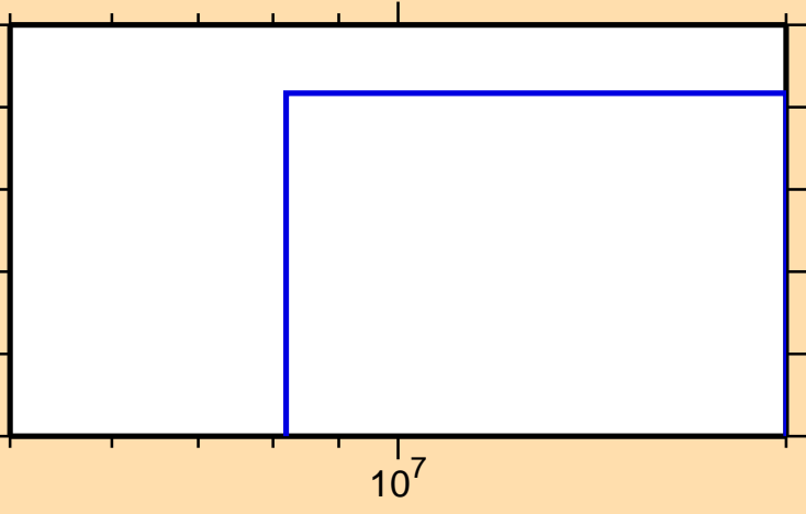
\sigma vs. E for ^{165}\text{W}(n,2np)
