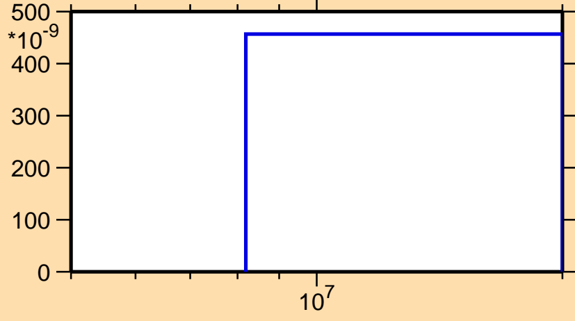
\sigma vs. E for ^{165}\text{W}(n,\text{pt})
