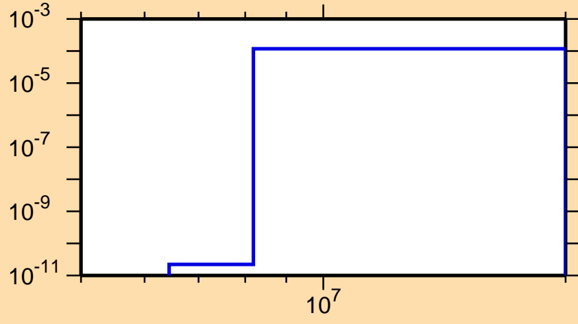
\sigma vs. E for ^{165}\text{W} (mt 45)
