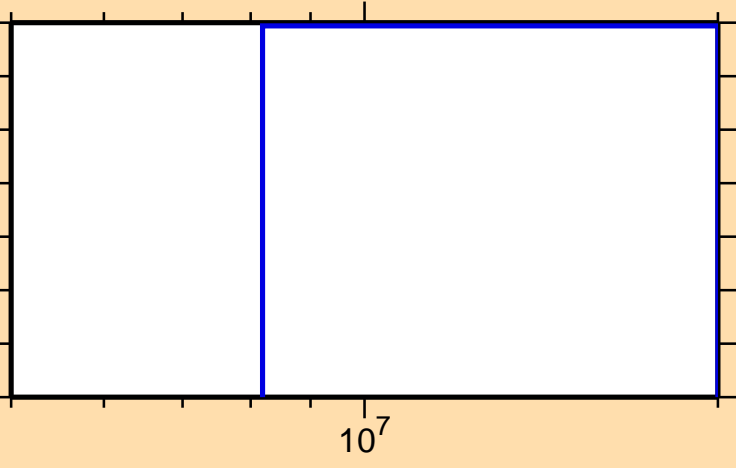
\sigma vs. E for ^{165}\text{W}(n,\text{pd})
