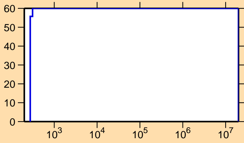
\Delta\sigma/\sigma vs. E for ^{166}\text{W}(n,\gamma)
