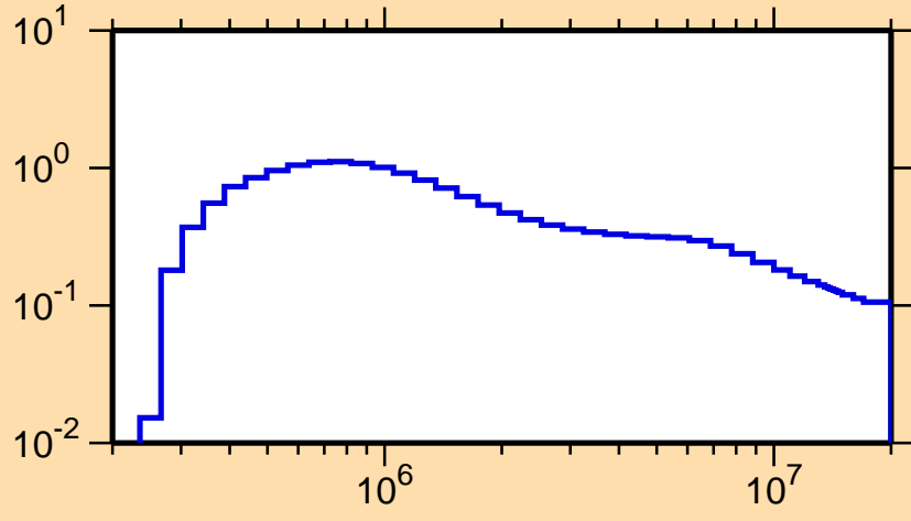
\sigma vs. E for ^{166}\text{W}(n,n_1)
