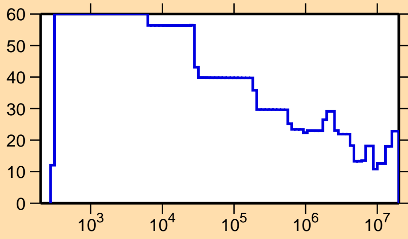
\Delta\sigma/\sigma vs. E for ^{166}\text{W}(n,\text{tot.})
