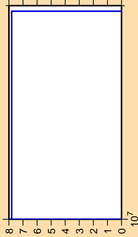
\Delta\sigma/\sigma vs. E for ^{166}\text{W} (mt 34)
