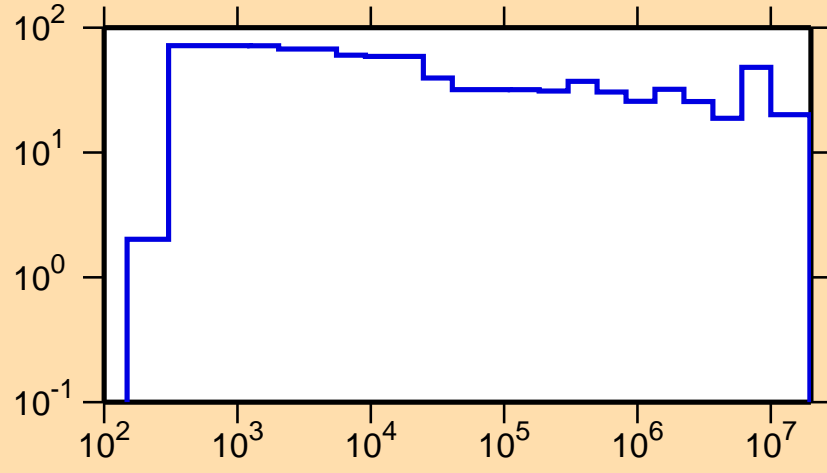
\Delta\sigma/\sigma vs. E for ^{166}\text{W}(n,el.)
