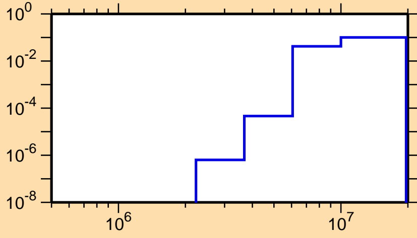
\sigma vs. E for ^{166}\text{W}(n,n\alpha)
