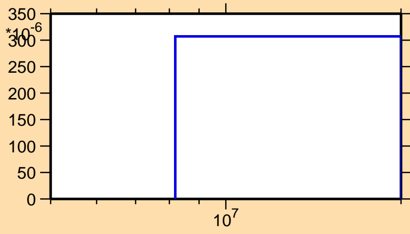
\sigma vs. E for ^{166}\text{W}(n,2n\alpha)
