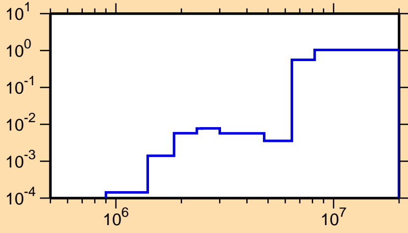
\sigma vs. E for ^{166}\text{W}(n,n\text{cont.})
