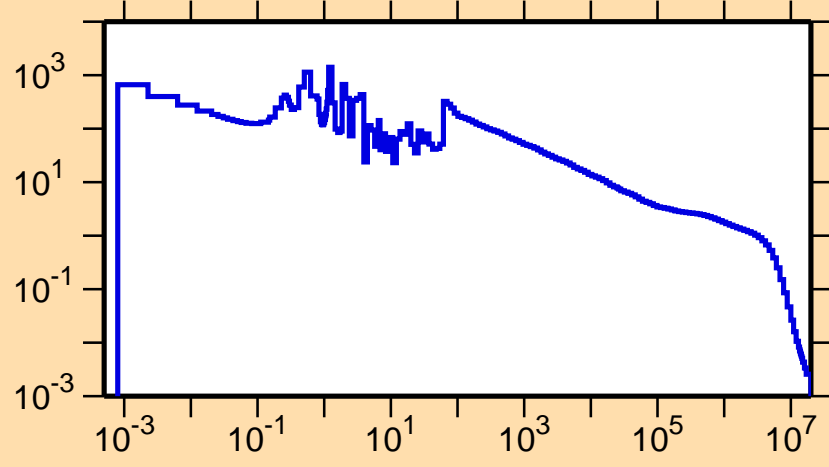
\sigma vs. E for ^{167}\text{W}(n,\gamma)
