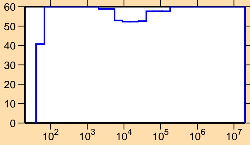
\Delta\sigma/\sigma vs. E for ^{167}\text{W}(n,\gamma)
