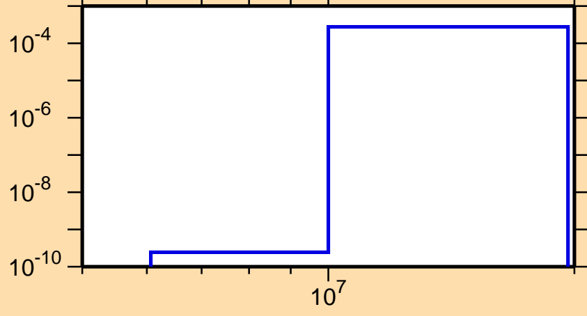
\sigma vs. E for ^{167}\text{W}(n,t)
