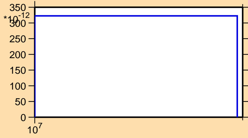
\sigma vs. E for ^{167}\text{W} (mt 34)
