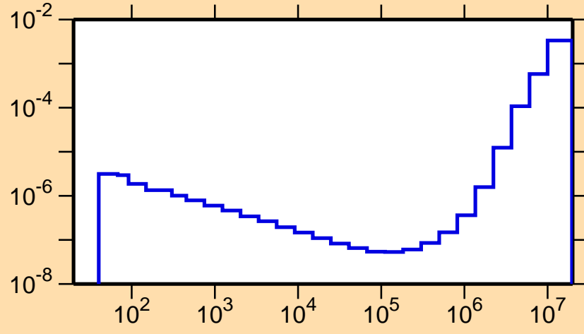
\sigma vs. E for ^{167}\text{W}(n,p\alpha)
