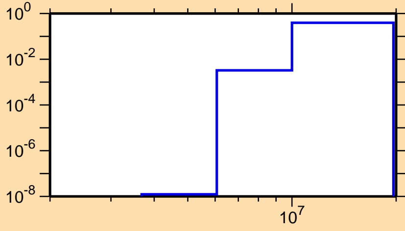
\sigma vs. E for ^{167}\text{W}(n,np)
