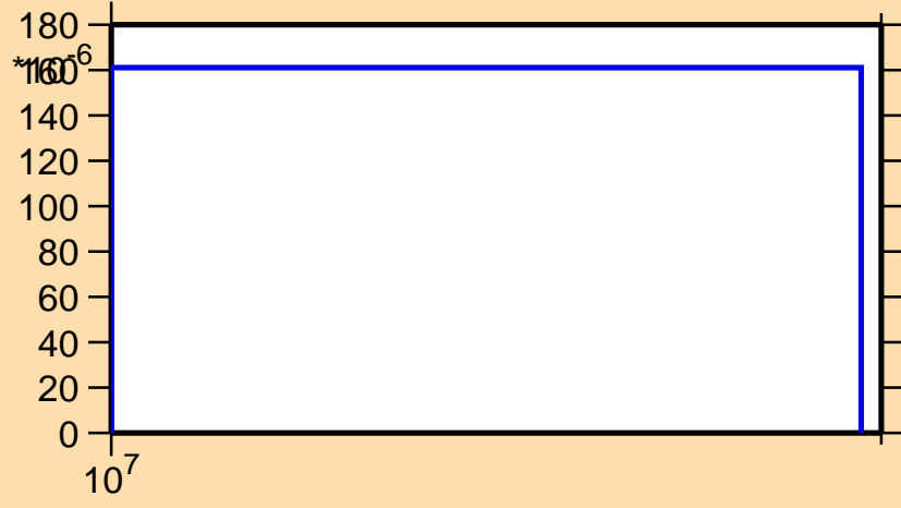
\sigma vs. E for ^{167}\text{W}(n,2np)
