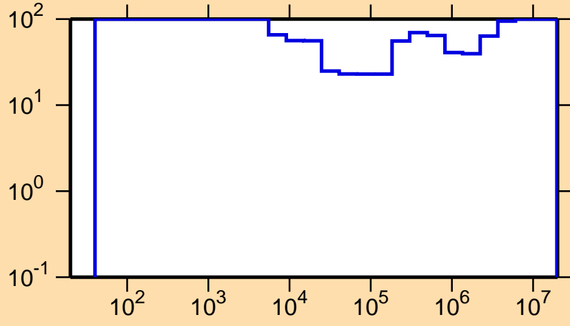
\Delta\sigma/\sigma vs. E for ^{167}\text{W}(n,el.)
