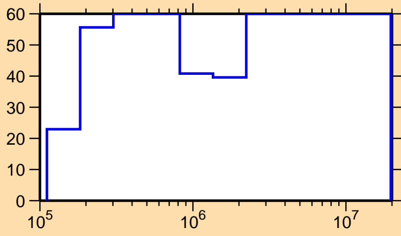
\Delta\sigma/\sigma vs. E for ^{167}\text{W}(n, el.)
