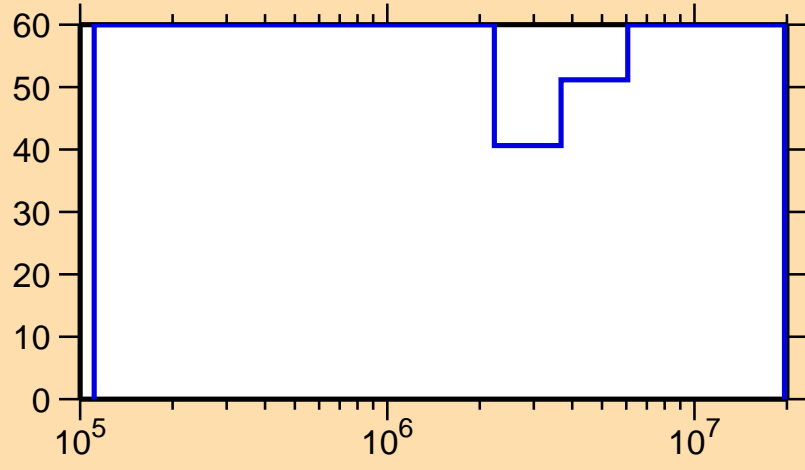
\Delta\sigma/\sigma vs. E for ^{167}\text{W}(n,\text{inel.})
