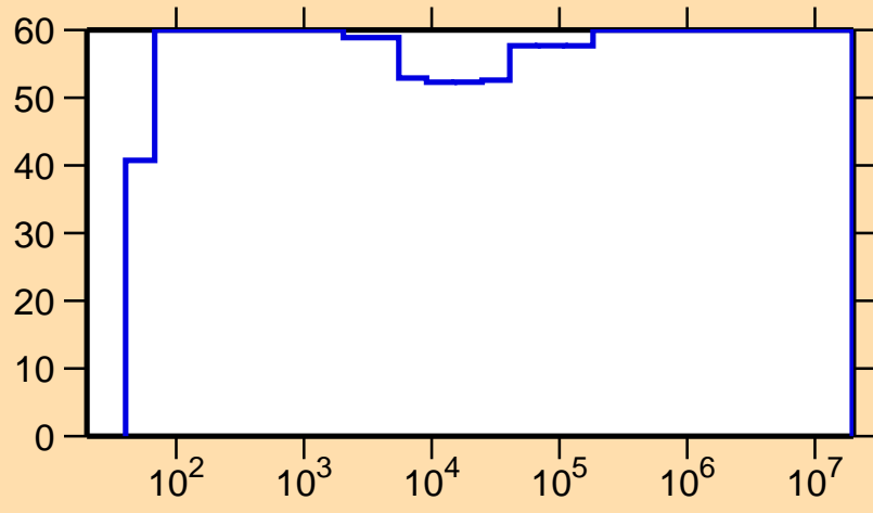
\Delta\sigma/\sigma vs. E for ^{167}\text{W}(n,\gamma)
