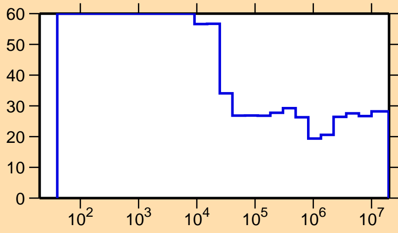
\Delta\sigma/\sigma vs. E for ^{167}\text{W}(n,\text{nonel.})
