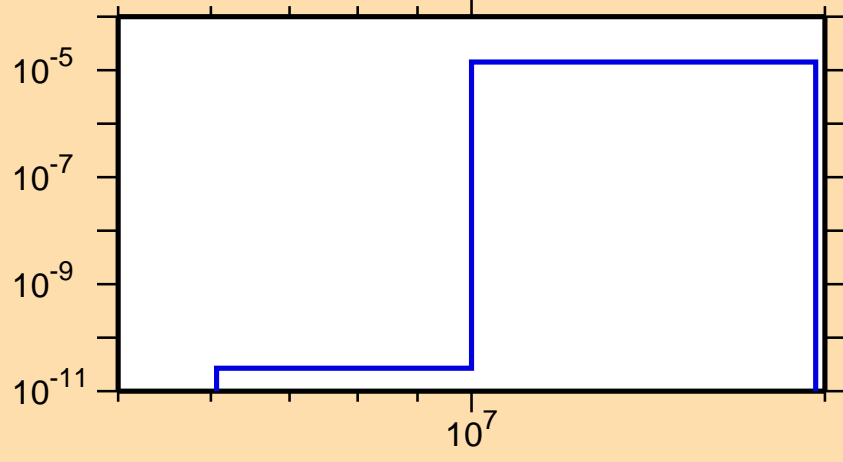
\sigma vs. E for ^{167}\text{W} (mt 45)
