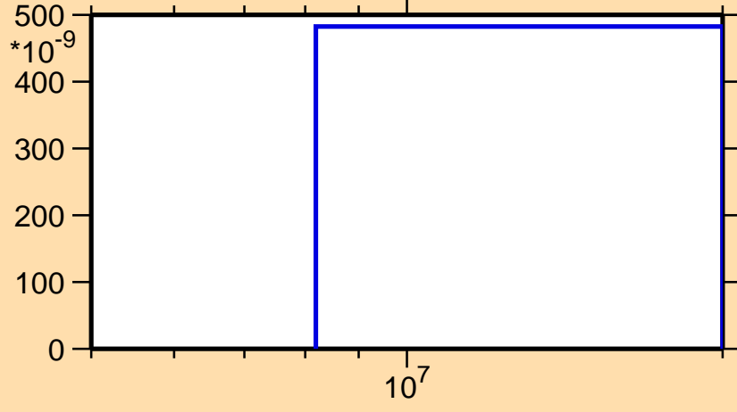
\sigma vs. E for ^{167}\text{W}(n,\text{pd})
