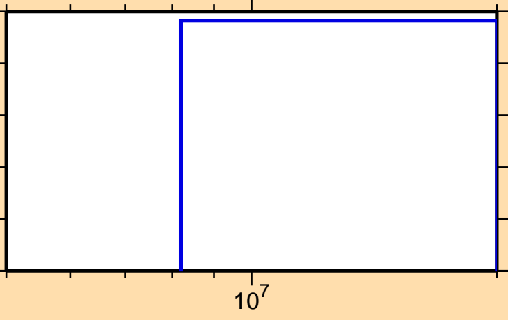
\sigma vs. E for ^{167}\text{W}(n,\text{pd})
