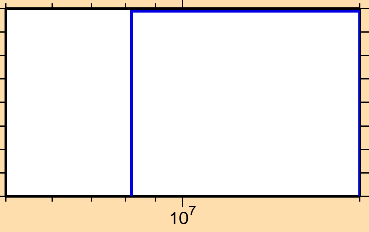
\sigma vs. E for ^{167}\text{W}(\text{mt117})
