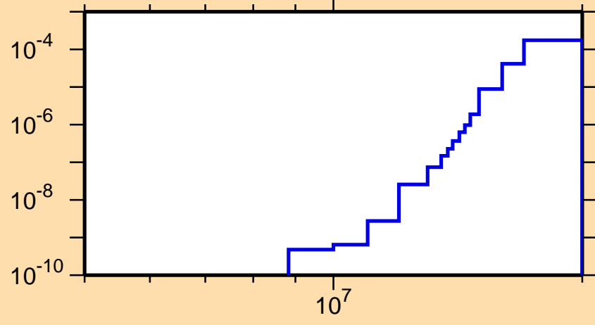
\sigma vs. E for ^{168}\text{W}(n,2n\alpha)
