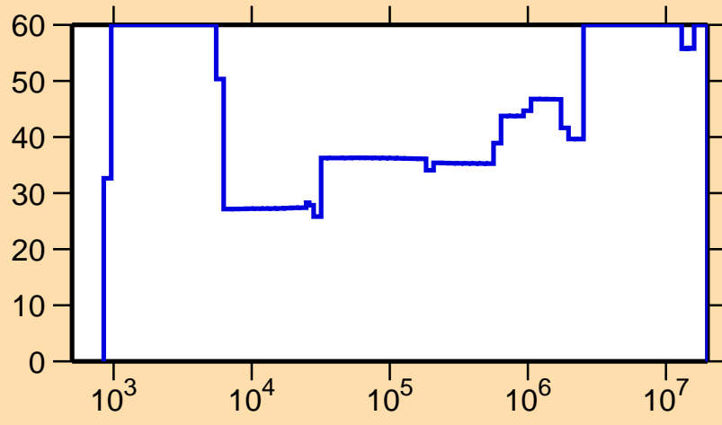
\Delta\sigma/\sigma vs. E for ^{168}\text{W}(n,\gamma)
