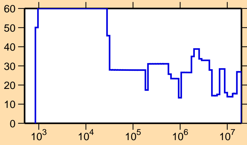
\Delta\sigma/\sigma vs. E for ^{168}\text{W}(n,el.)
