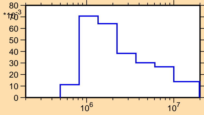
\sigma vs. E for ^{168}\text{W}(n,n_2)
