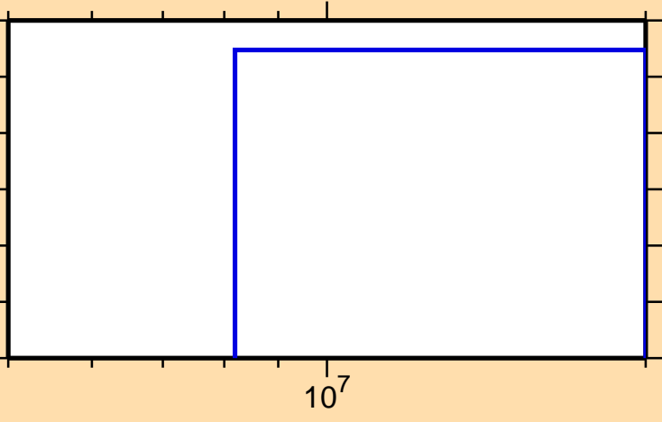
\sigma vs. E for ^{168}\text{W}(\text{mt117})
