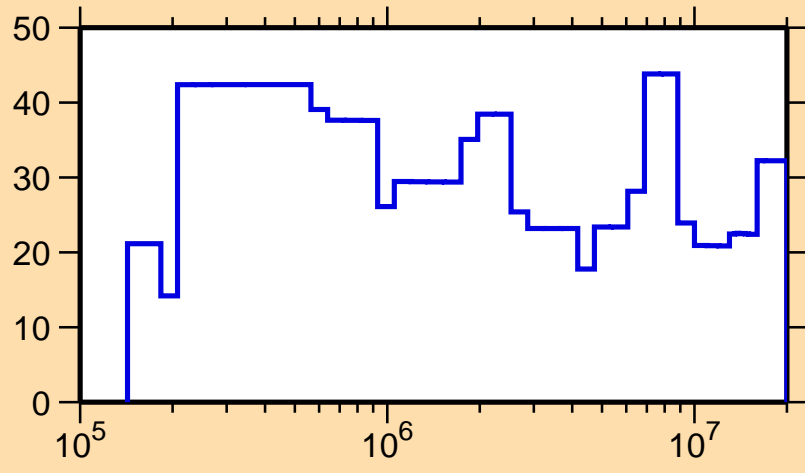
\Delta\sigma/\sigma vs. E for ^{169}\text{W}(n, el.)
