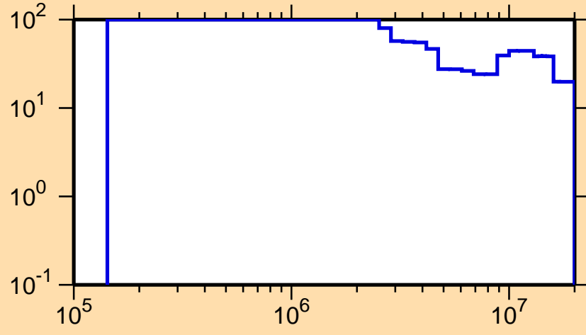
\Delta\sigma/\sigma vs. E for ^{169}\text{W}(n, inel.)
