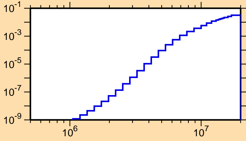
\sigma vs. E for ^{169}\text{W}(n,n\alpha)
