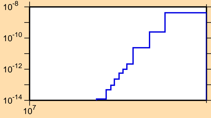
\sigma vs. E for ^{169}\text{W} (mt 34)
