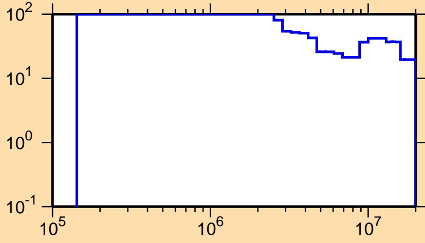
\Delta\sigma/\sigma vs. E for ^{169}\text{W}(n,ncont.)
