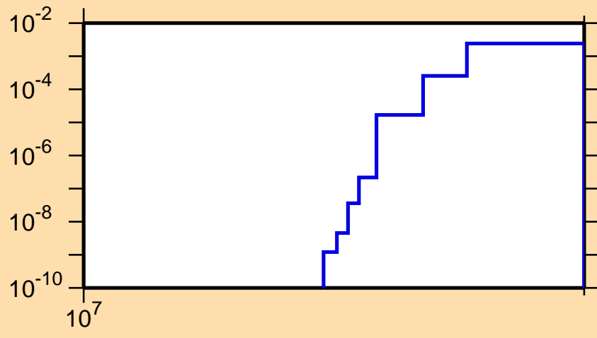
\sigma vs. E for ^{169}\text{W}(n,2np)
