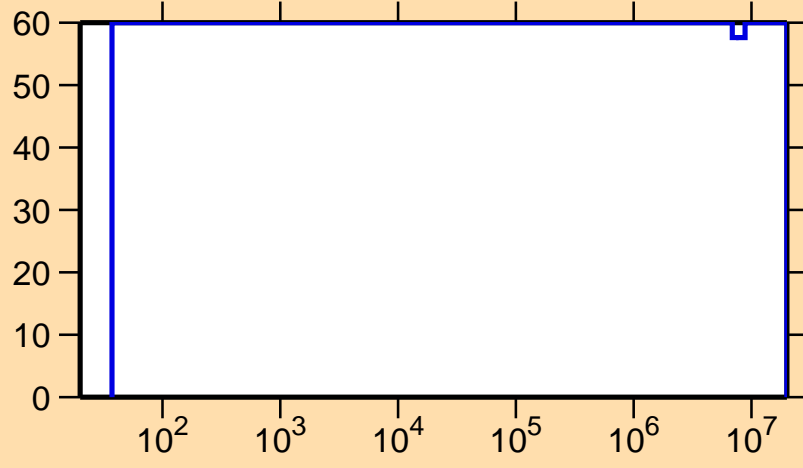
\Delta\sigma/\sigma vs. E for ^{169}\text{W}(n,p)
