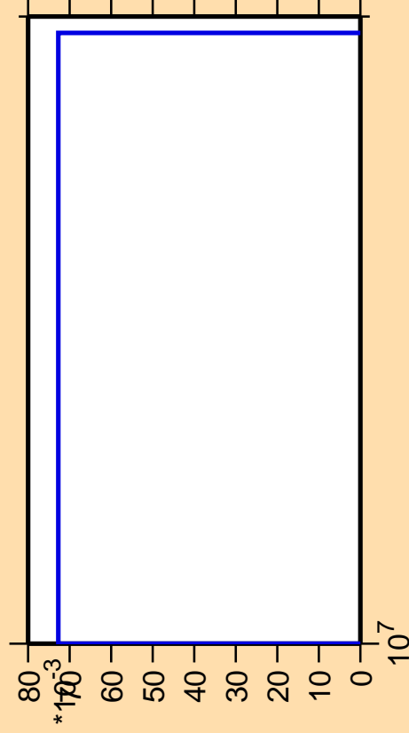
\Delta\sigma/\sigma vs. E for ^{169}\text{W}(n,3n\alpha)
