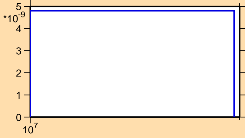
\sigma vs. E for ^{169}\text{W}(n,\text{pt})
