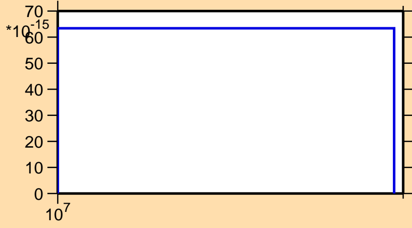
\sigma vs. E for ^{169}\text{W}(n,3n\alpha)
