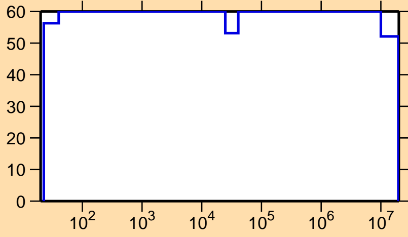
\Delta\sigma/\sigma vs. E for ^{169}\text{W}(n,\gamma)
