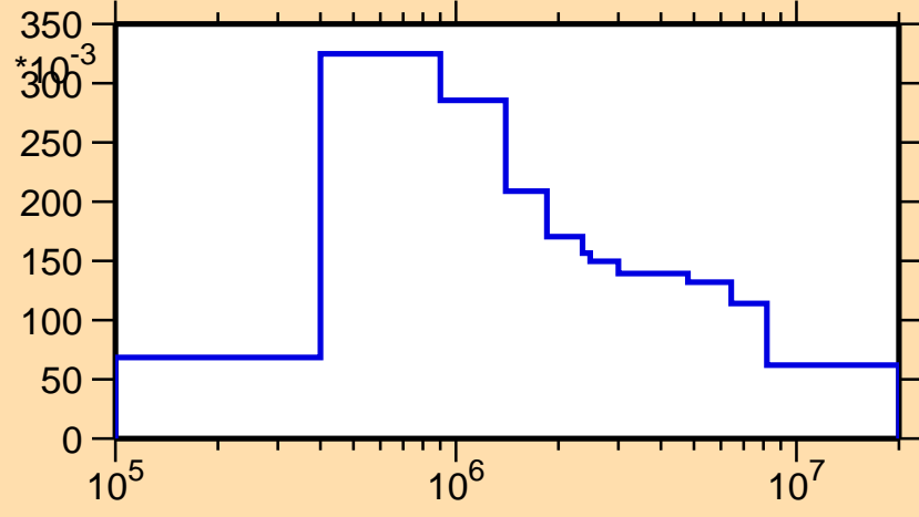
\sigma vs. E for ^{169}\text{W}(n,n_1)
