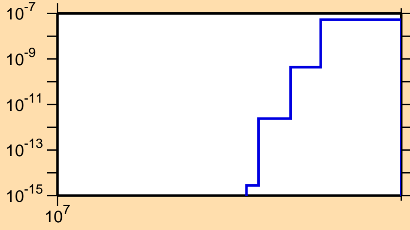
\sigma vs. E for ^{170}\text{W}(n,\text{nd})
