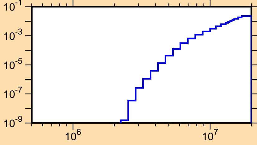
\sigma vs. E for ^{170}\text{W}(n,n\alpha)
