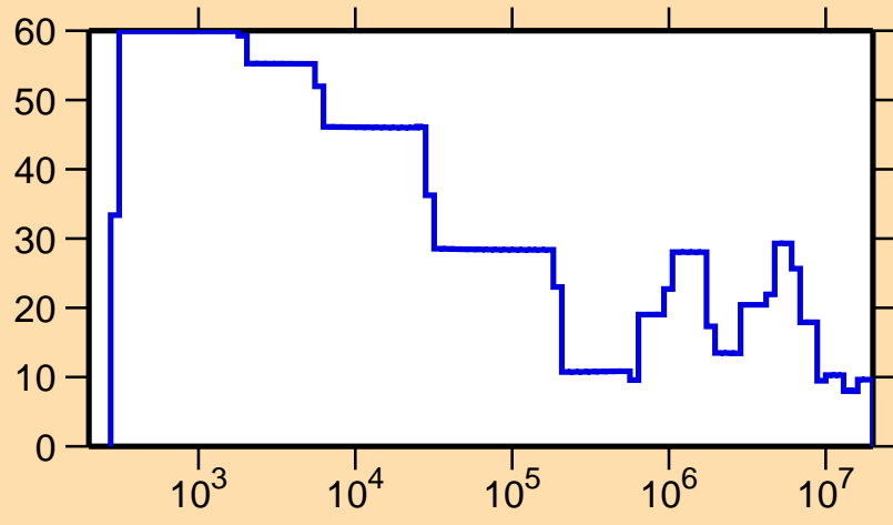
\Delta\sigma/\sigma vs. E for ^{170}\text{W}(n,el.)
