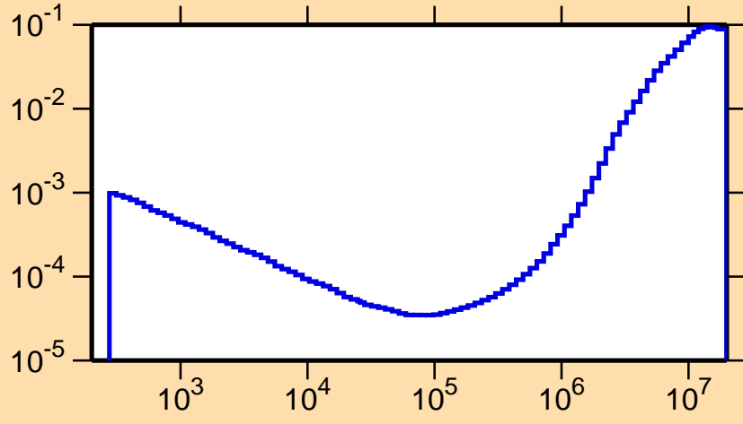
\sigma vs. E for ^{170}\text{W}(n,p)
