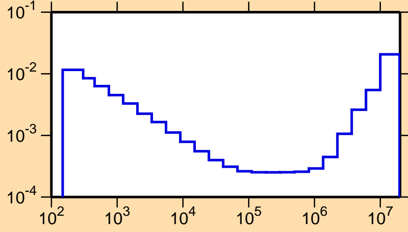
\sigma vs. E for ^{170}\text{W}(n,\alpha)
