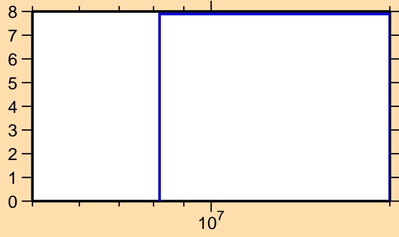
\Delta\sigma/\sigma vs. E for ^{170}\text{W}(n,\text{el.})
