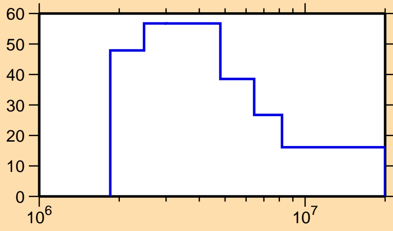
\Delta\sigma/\sigma vs. E for ^{170}\text{W}(n,ncont.)
