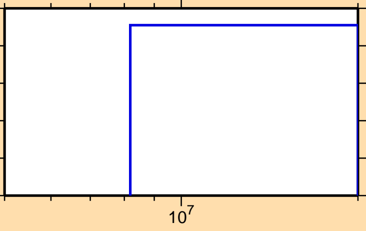
\sigma vs. E for ^{170}\text{W}(n,3n)
