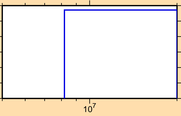
\sigma vs. E for ^{170}\text{W}(\text{mt117})
