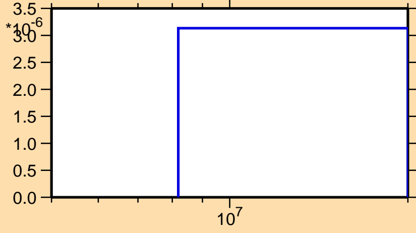
\sigma vs. E for ^{170}\text{W}(n,2n\alpha)
