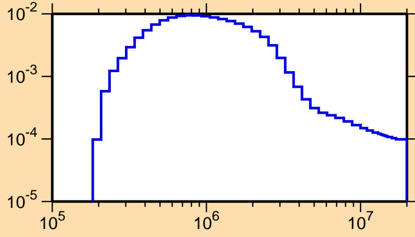
\sigma vs. E for ^{171}\text{W}(n,n_3)
