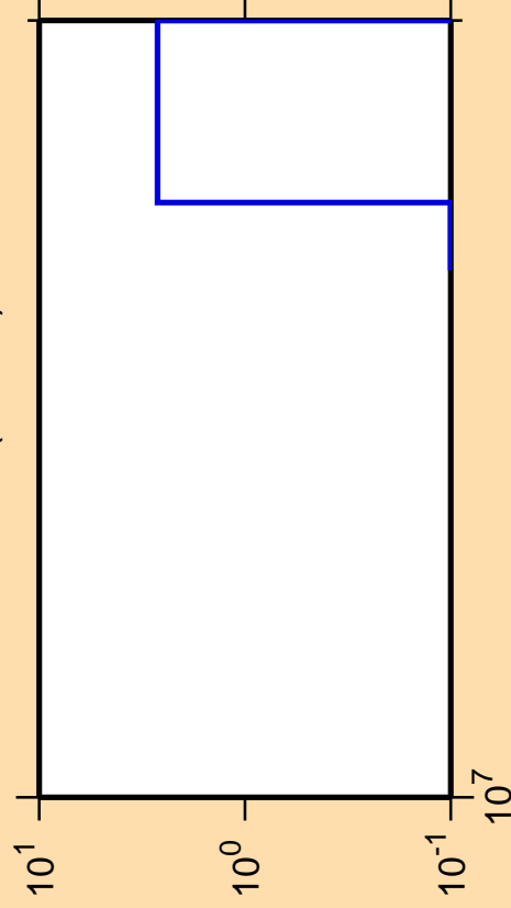
\Delta\sigma/\sigma vs. E for ^{171}\text{W}(n,3n\alpha)
