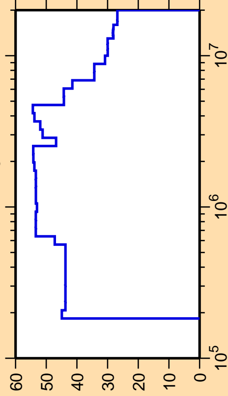
\Delta\sigma/\sigma vs. E for ^{171}\text{W}(n,n_3)
