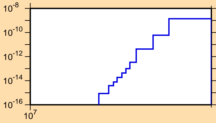
\sigma vs. E for ^{171}\text{W} (mt 34)
