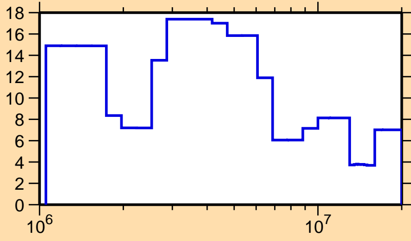
\Delta\sigma/\sigma vs. E for ^{171}\text{W}(n, el.)
