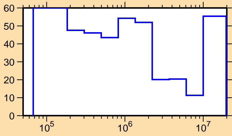
\Delta\sigma/\sigma vs. E for ^{171}\text{W}(n,\text{inel.})
