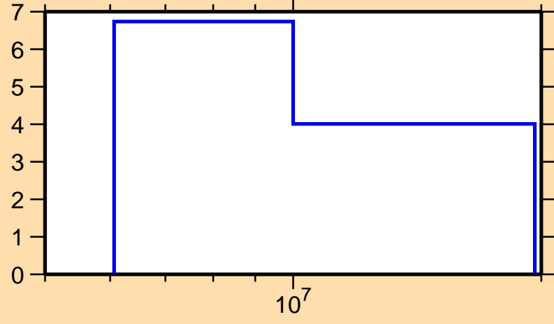
\Delta\sigma/\sigma vs. E for ^{171}\text{W}(n,\text{el.})
