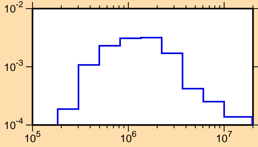
\sigma vs. E for ^{171}\text{W}(n,n_4)
