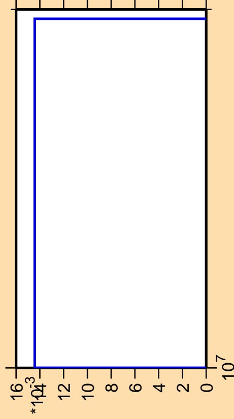
\Delta\sigma/\sigma vs. E for ^{171}\text{W}(n,3n\alpha)
