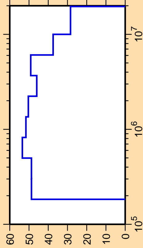
\Delta\sigma/\sigma vs. E for ^{171}\text{W}(n,n_4)
