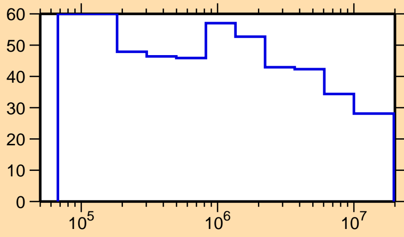
\Delta\sigma/\sigma vs. E for ^{171}\text{W}(n,n_1)
