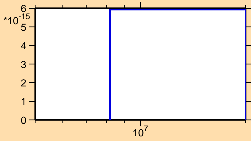
\sigma vs. E for ^{171}\text{W}(n,3n\alpha)
