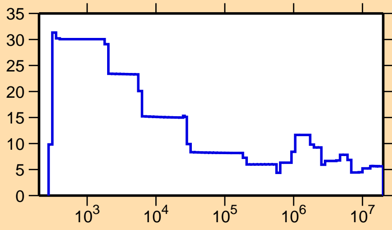
\Delta\sigma/\sigma vs. E for ^{172}\text{W}(n,el.)
