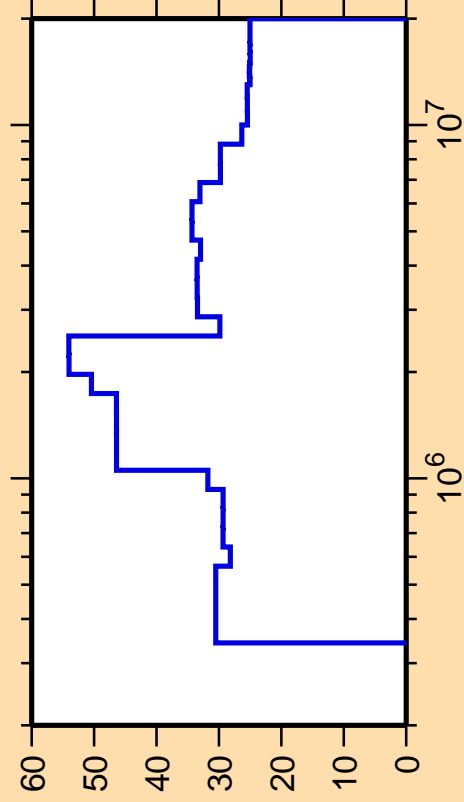
\Delta\sigma/\sigma vs. E for ^{172}\text{W}(n,n_2)
