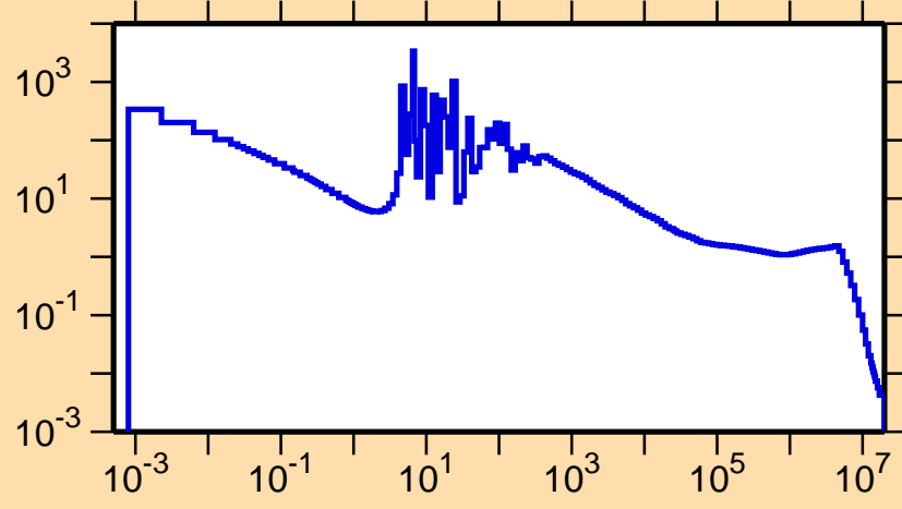
\sigma vs. E for ^{172}\text{W}(n,\gamma)
