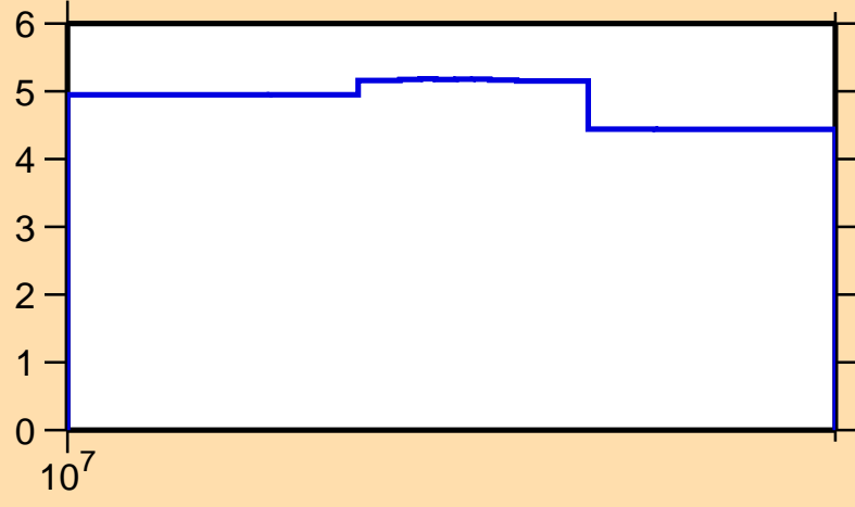
\Delta\sigma/\sigma vs. E for ^{172}\text{W}(n,\text{nonel.})
