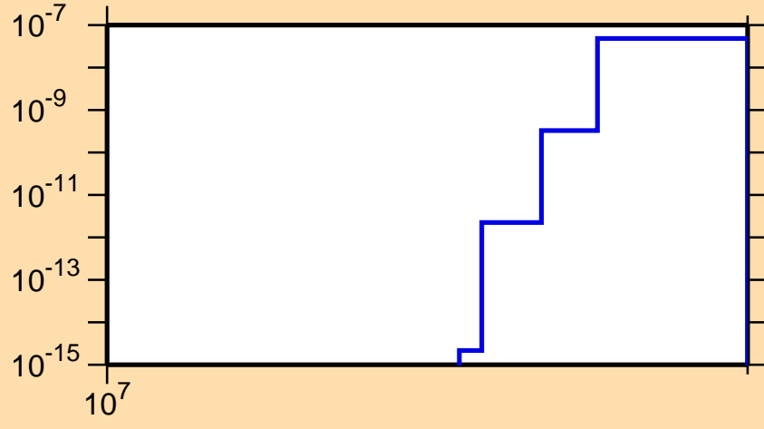
\sigma vs. E for ^{172}\text{W}(n,\text{nd})
