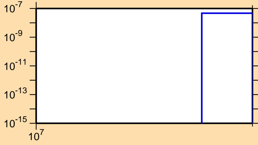
\sigma vs. E for ^{172}\text{W}(n,3n\alpha)
