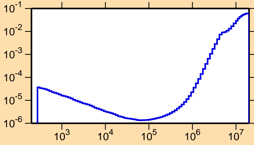
\sigma vs. E for ^{172}\text{W}(n,p)
