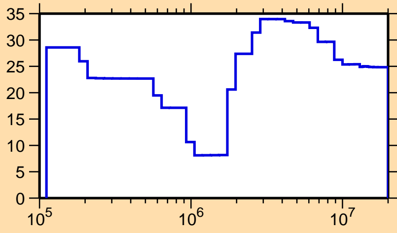
\Delta\sigma/\sigma vs. E for ^{172}\text{W}(n,n_1)
