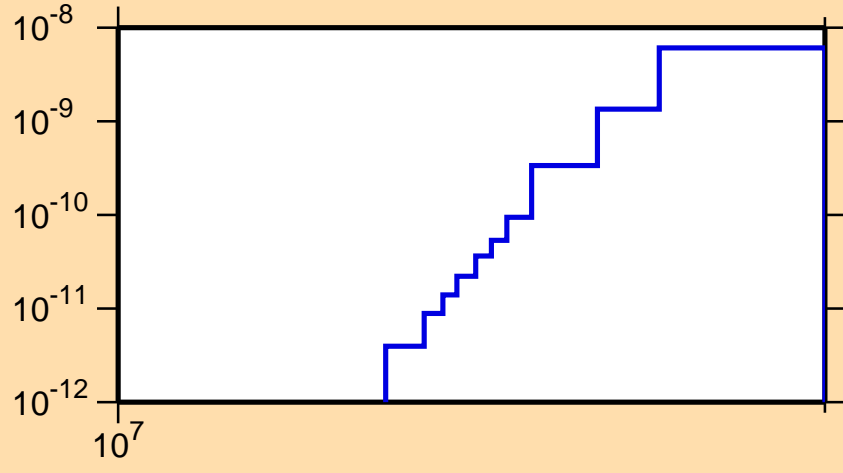
\sigma vs. E for ^{172}\text{W}(\text{mt117})
