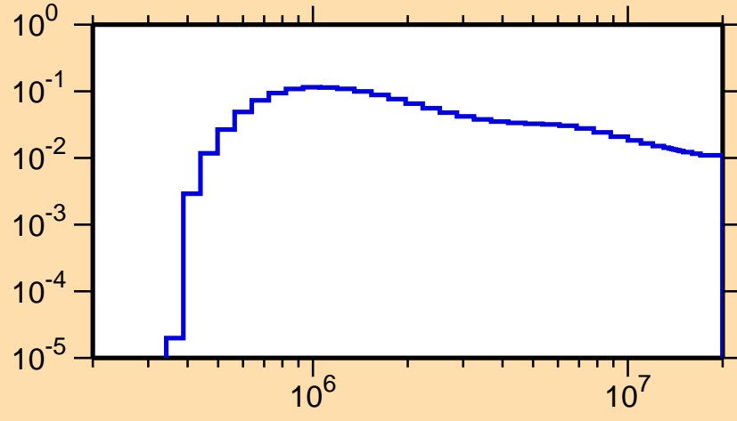
\sigma vs. E for ^{172}\text{W}(n,n_2)
