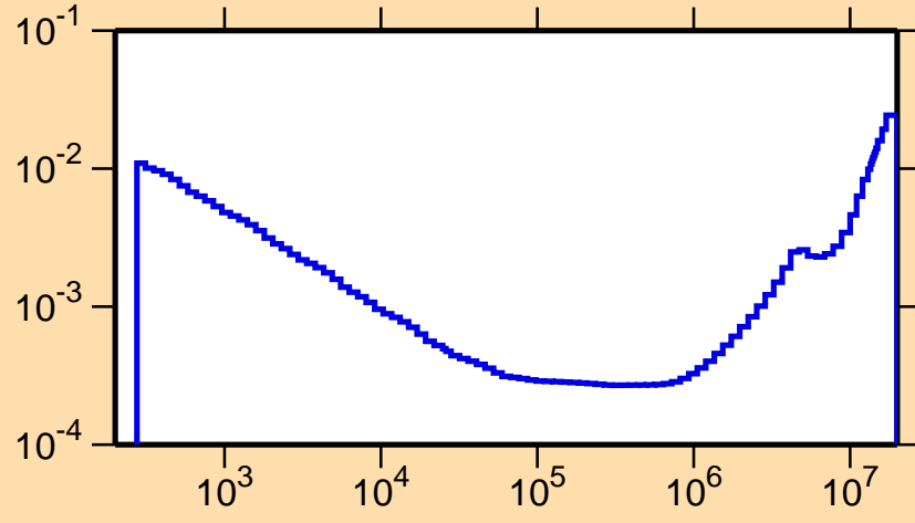
\sigma vs. E for ^{172}\text{W}(n,\alpha)
