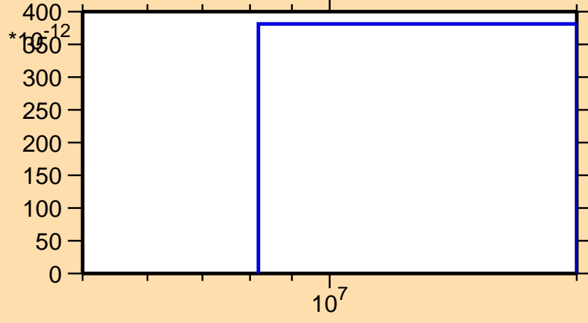
\sigma vs. E for ^{172}\text{W}(n,3n\alpha)
