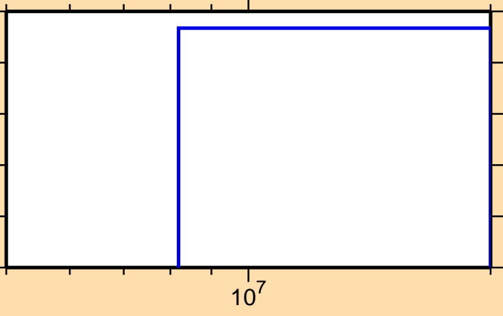
\sigma vs. E for ^{172}\text{W}(n,3n)
