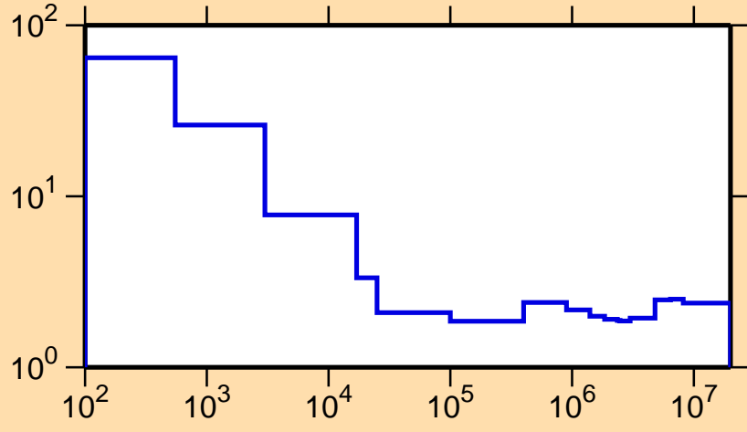
\sigma vs. E for ^{172}\text{W}(n,\text{nonel.})
