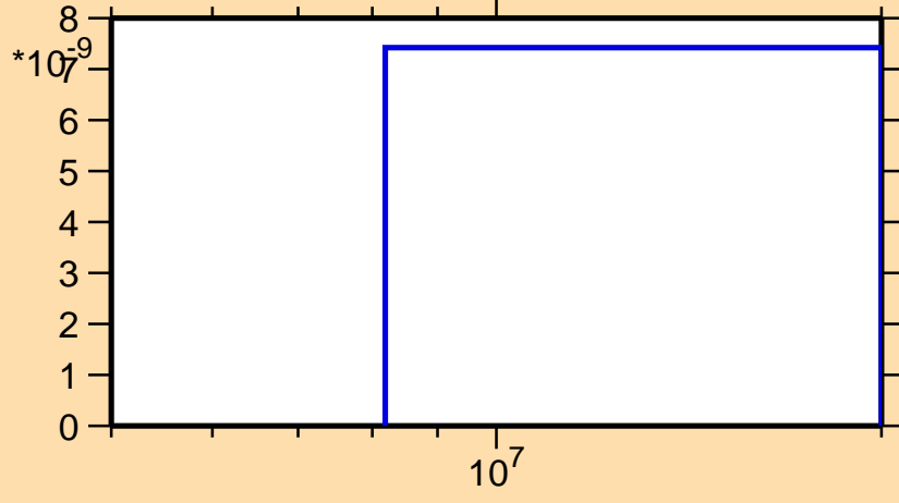
\sigma vs. E for ^{172}\text{W} (mt 45)
