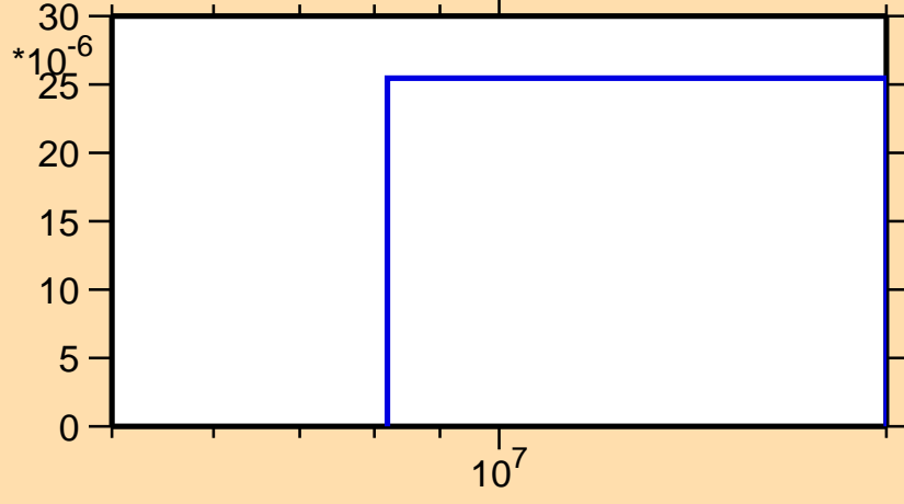
\sigma vs. E for ^{172}\text{W}(n,t)
