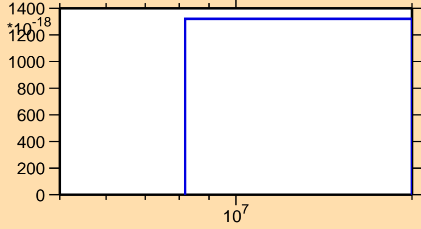
\sigma vs. E for ^{173}\text{W}(n,3n\alpha)
