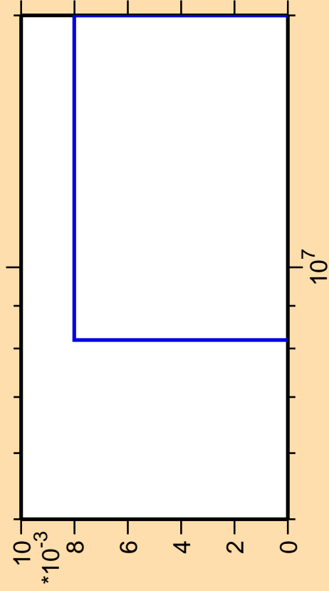
\Delta\sigma/\sigma vs. E for ^{173}\text{W}(n,3n\alpha)
