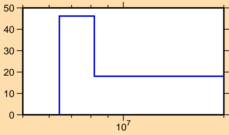
\Delta\sigma/\sigma vs. E for ^{173}\text{W}(n,2n)
