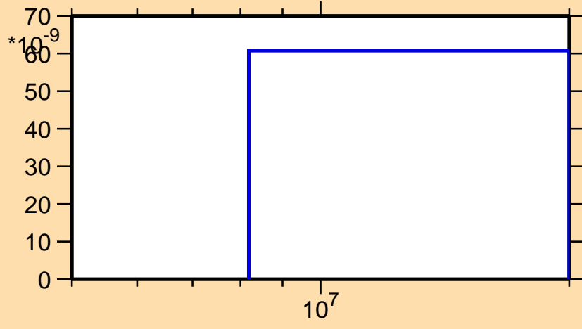
\sigma vs. E for ^{173}\text{W}(n,\text{nd})
