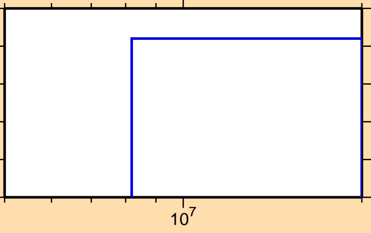
\sigma vs. E for ^{173}\text{W}(n,3n)
