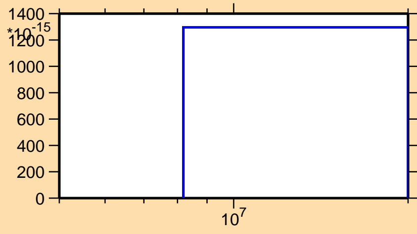
\sigma vs. E for ^{173}\text{W}(n,nt)
