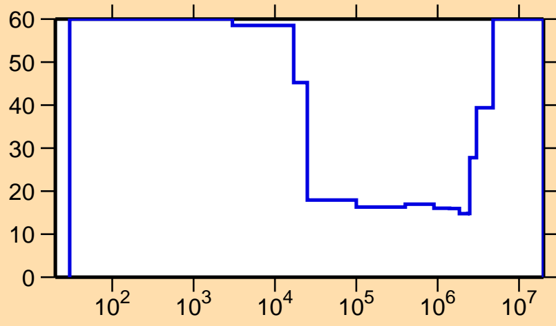
\Delta\sigma/\sigma vs. E for ^{173}\text{W}(n,\gamma)
