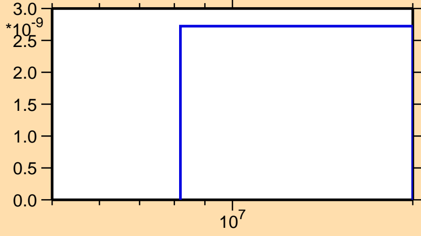
\sigma vs. E for ^{173}\text{W} (mt 45)
