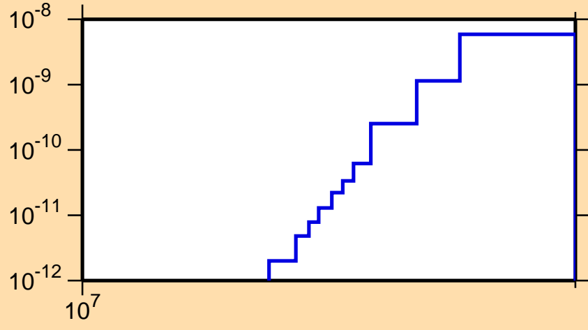
\sigma vs. E for ^{174}\text{W}(\text{mt117})
