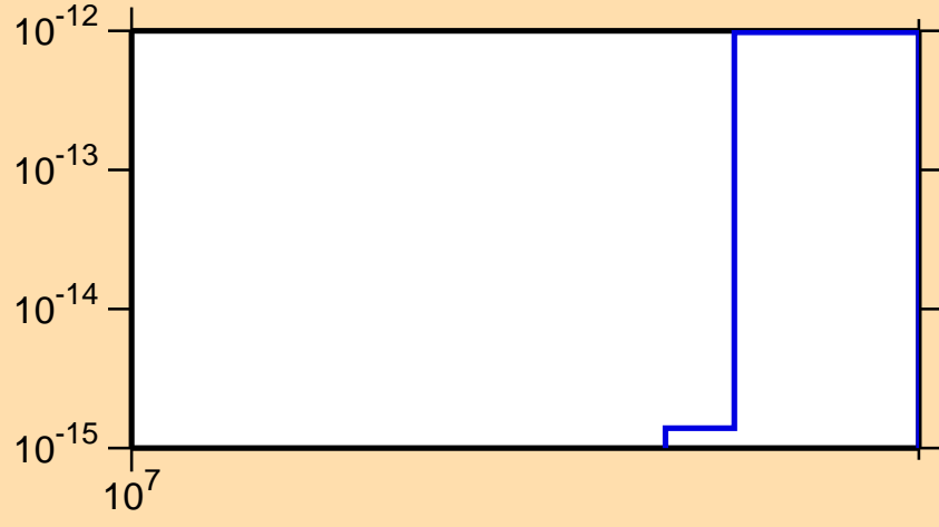
\sigma vs. E for ^{174}\text{W} (mt 34)
