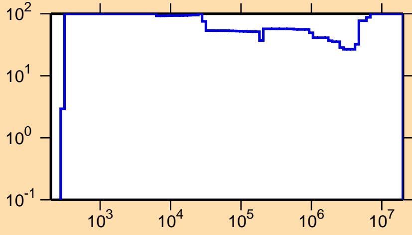
\Delta\sigma/\sigma vs. E for ^{174}\text{W}(n,\gamma)
