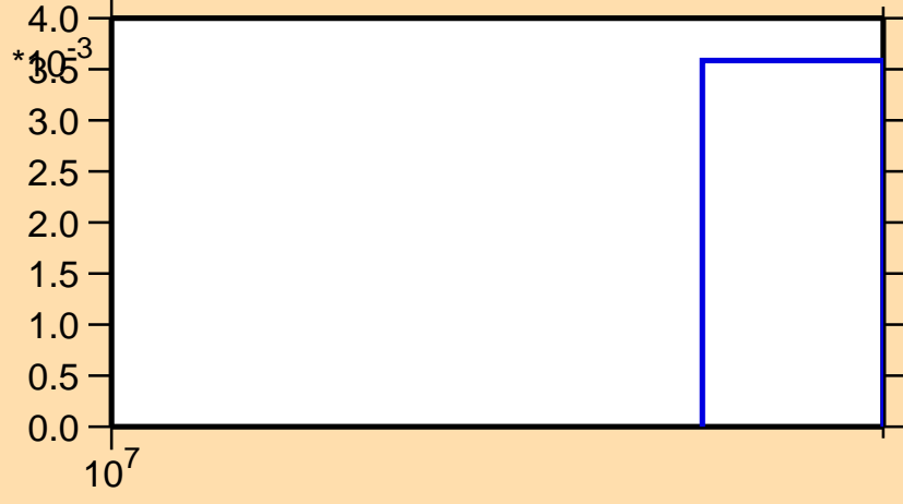
\sigma vs. E for ^{174}\text{W}(n,3n)
