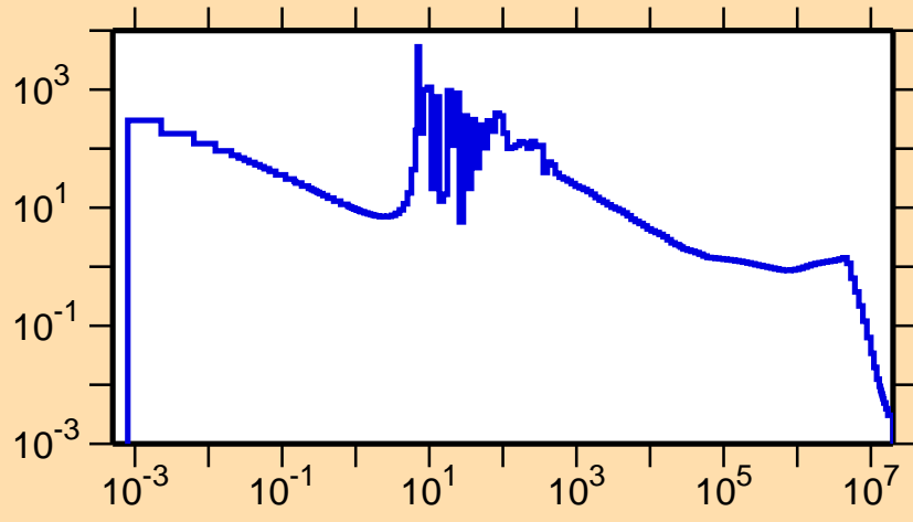
\sigma vs. E for ^{174}\text{W}(n,\gamma)
