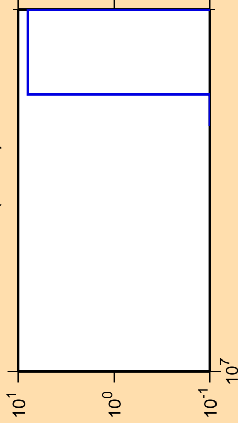
\Delta\sigma/\sigma vs. E for ^{174}\text{W} (mt 34)
