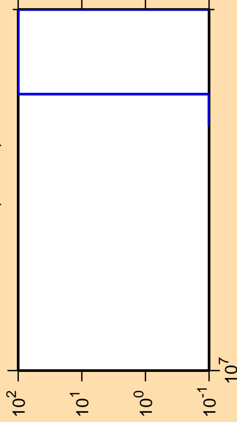
\Delta\sigma/\sigma vs. E for ^{174}\text{W}(n,3n\alpha)
