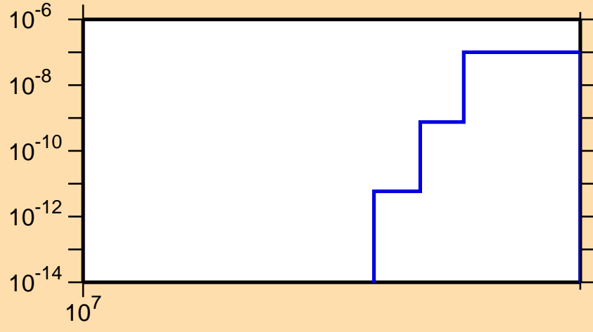
\sigma vs. E for ^{174}\text{W}(n,\text{nd})
