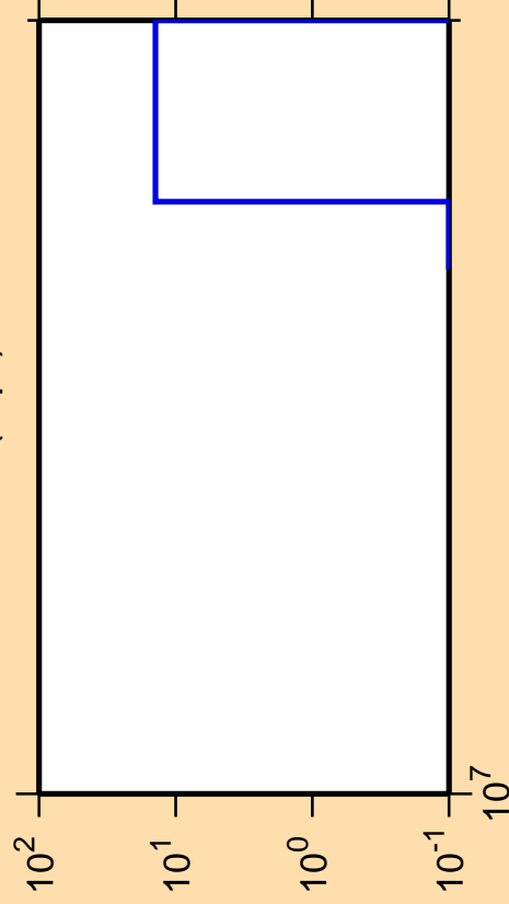
\Delta\sigma/\sigma vs. E for ^{174}\text{W}(n,\text{pt})
