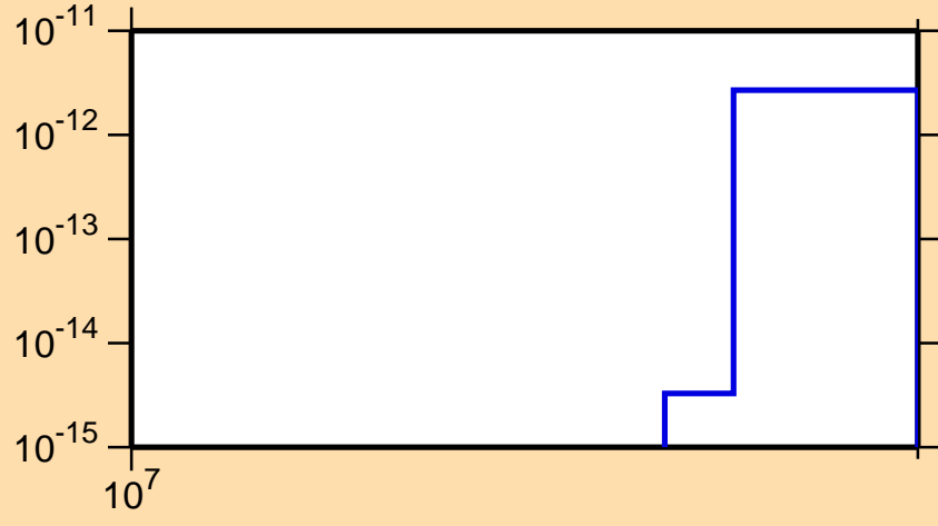
\sigma vs. E for ^{174}\text{W}(n,\text{pt})
