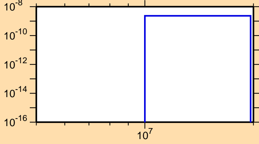
\sigma vs. E for ^{174}\text{W} (mt 45)
