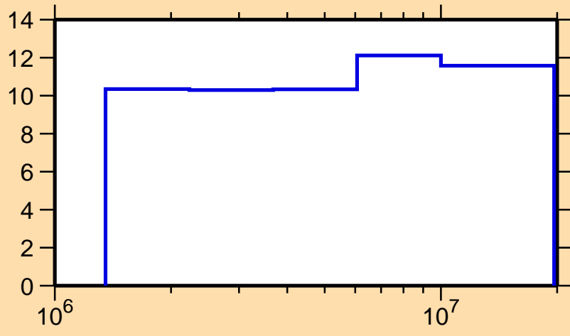
\Delta\sigma/\sigma vs. E for ^{174}\text{W}(n,tot.)
