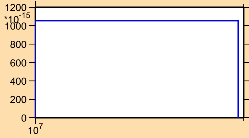
\sigma vs. E for ^{174}\text{W}(n,3n\alpha)
