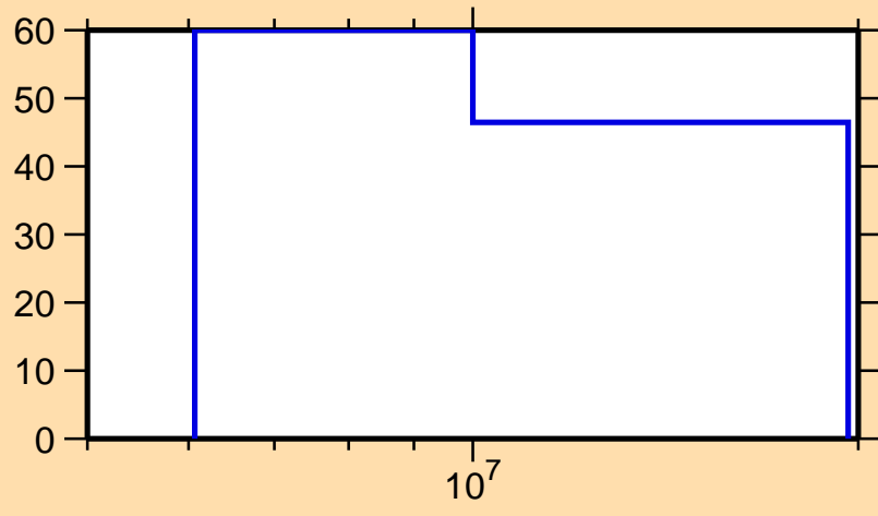
\Delta\sigma/\sigma vs. E for ^{174}\text{W}(n,2n)
