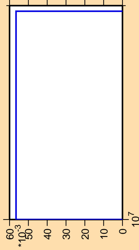
\Delta\sigma/\sigma vs. E for ^{174}\text{W} (mt 34)
