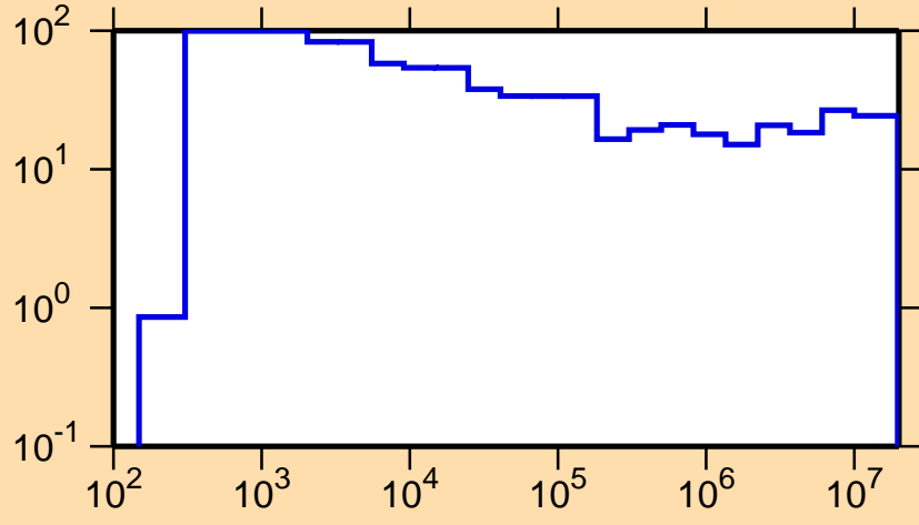
\Delta\sigma/\sigma vs. E for ^{174}\text{W}(n,el.)
