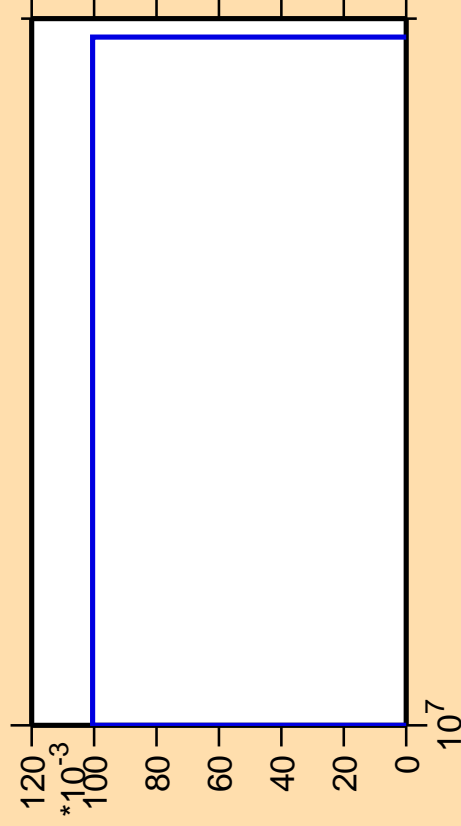
\Delta\sigma/\sigma vs. E for ^{174}\text{W}(n,\text{pt})
