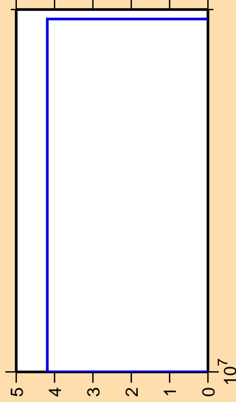
\Delta\sigma/\sigma vs. E for ^{174}\text{W}(n,3n\alpha)
