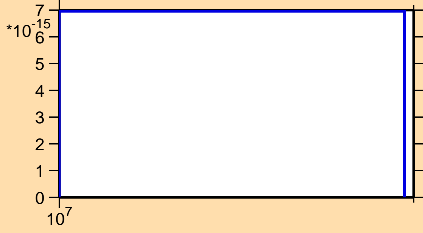
\sigma vs. E for ^{174}\text{W} (mt 34)
