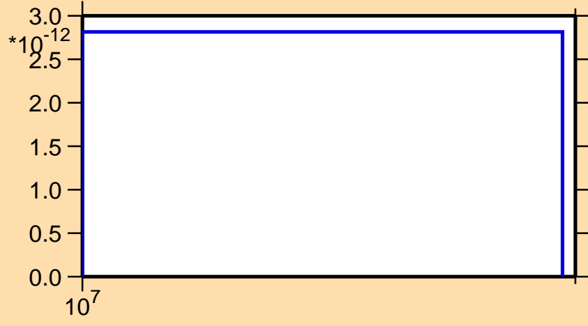
\sigma vs. E for ^{174}\text{W}(n,nt)
