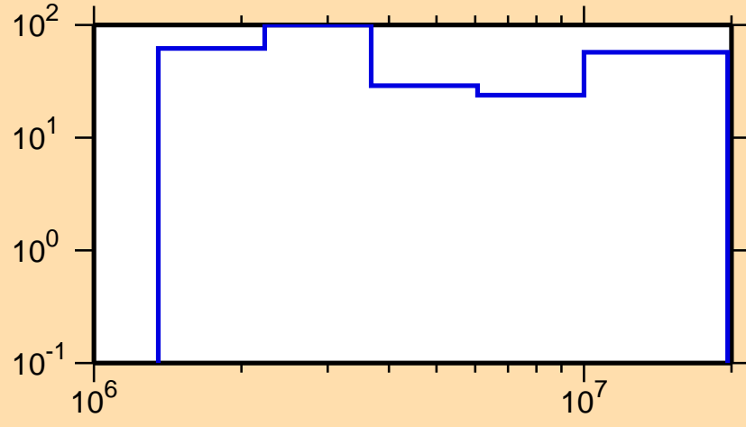
\Delta\sigma/\sigma vs. E for ^{174}\text{W}(n,n\text{cont.})
