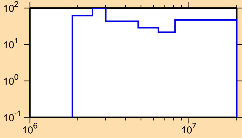
\Delta\sigma/\sigma vs. E for ^{174}\text{W}(n,ncont.)
