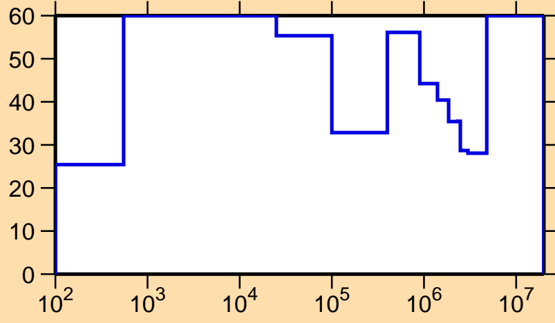
\Delta\sigma/\sigma vs. E for ^{174}\text{W}(n,\gamma)
