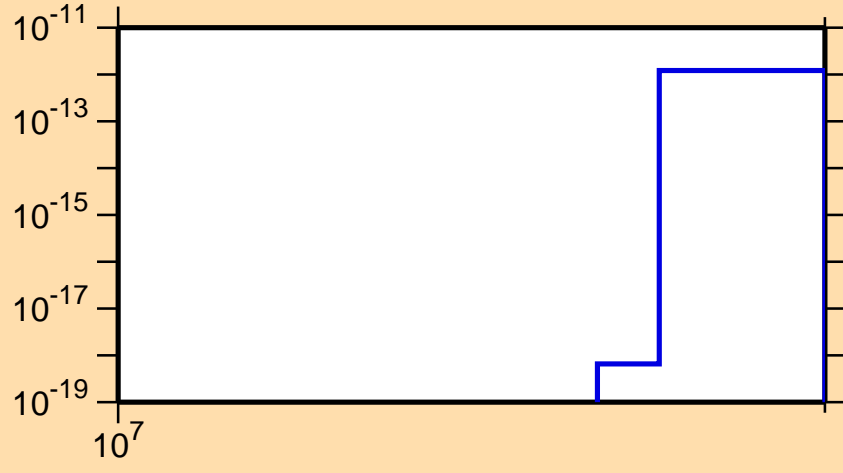
\sigma vs. E for ^{175}\text{W}(n,3n\alpha)
