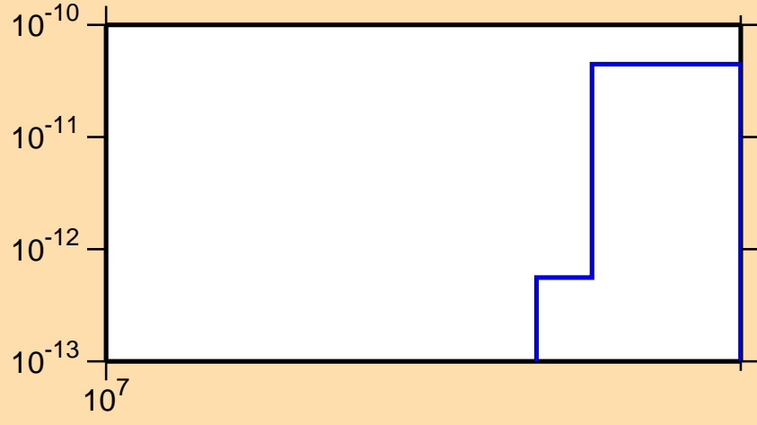
\sigma vs. E for ^{175}\text{W} (mt 34)
