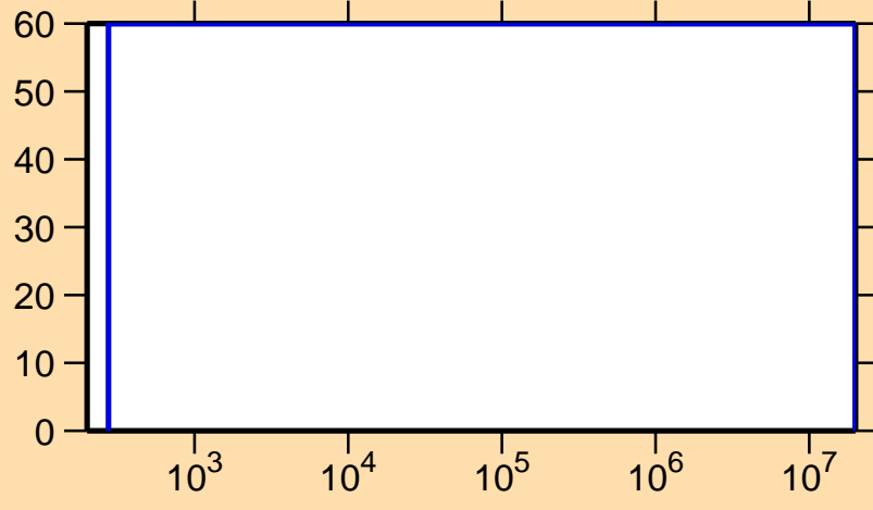
\Delta\sigma/\sigma vs. E for ^{175}\text{W}(n,p)
