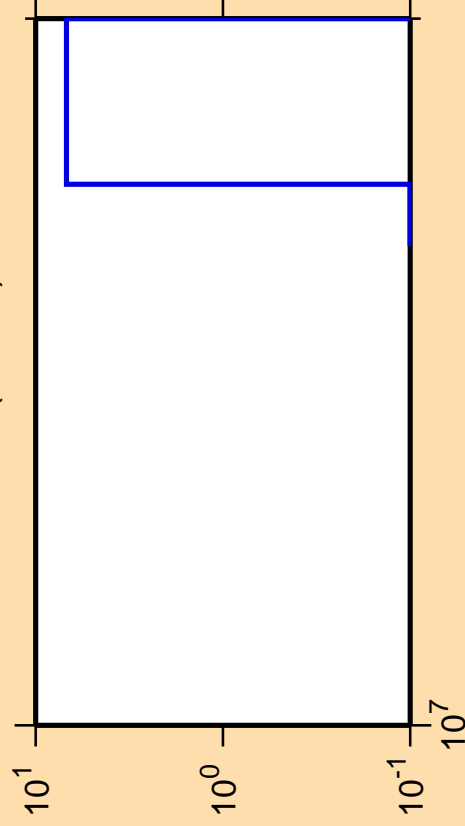
\Delta\sigma/\sigma vs. E for ^{175}\text{W}(n,3n\alpha)
