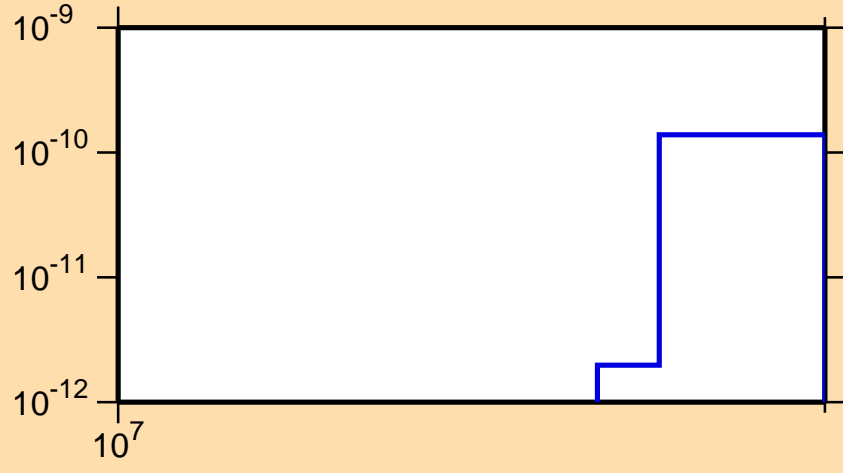
\sigma vs. E for ^{175}\text{W}(n,\text{pt})
