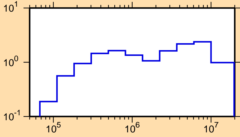
\sigma vs. E for ^{175}\text{W}(n,\text{inel.})
