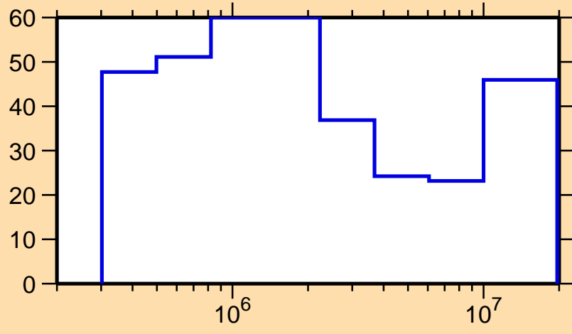
\Delta\sigma/\sigma vs. E for ^{175}\text{W}(n,n\text{cont.})
