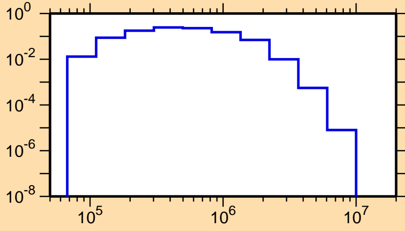
\sigma vs. E for ^{175}\text{W}(n,n_2)
