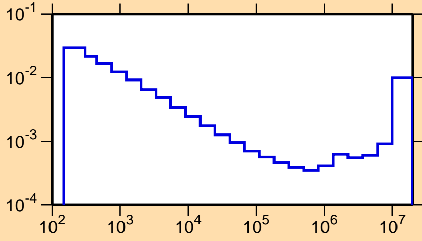
\sigma vs. E for ^{175}\text{W}(n,\alpha)
