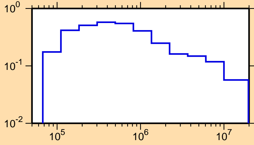
\sigma vs. E for ^{175}\text{W}(n,n_1)
