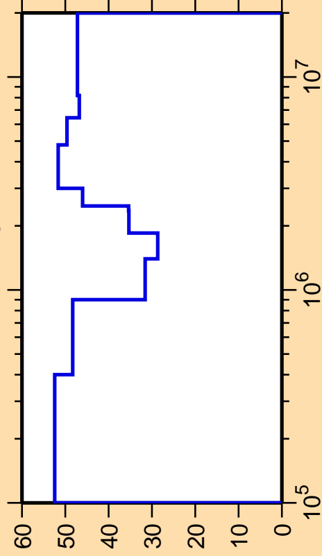
\Delta\sigma/\sigma vs. E for ^{175}\text{W}(n,n_3)
