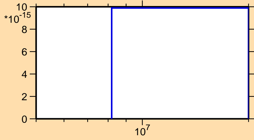
\sigma vs. E for ^{175}\text{W}(n,3n\alpha)
