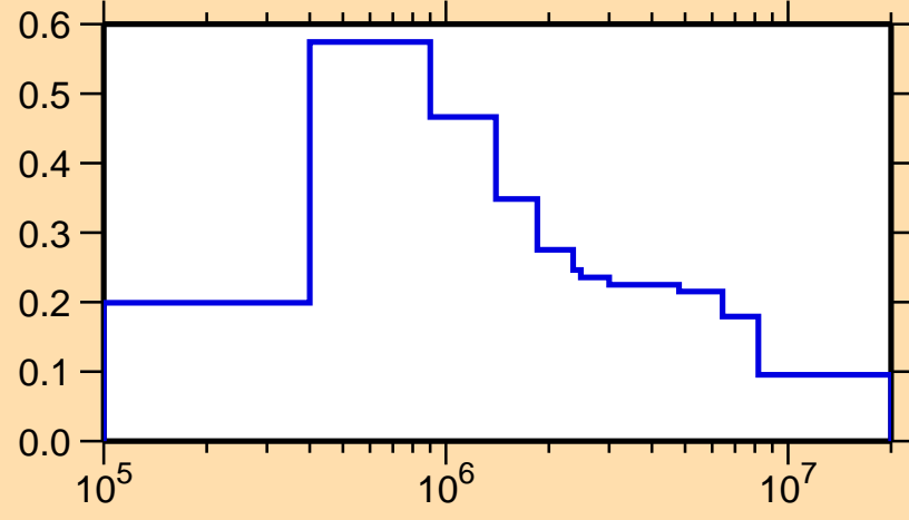
\sigma vs. E for ^{175}\text{W}(n,n_3)
