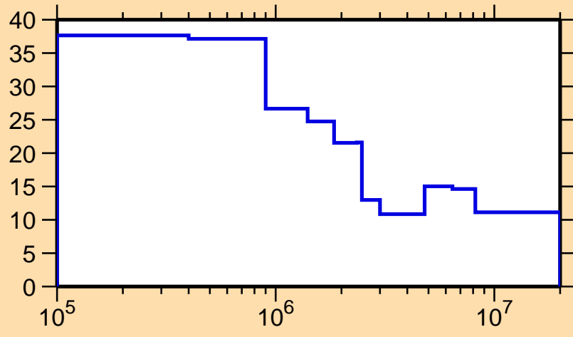
\Delta\sigma/\sigma vs. E for ^{175}\text{W}(n, nonel.)
