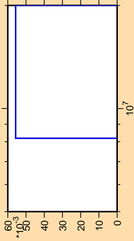
\Delta\sigma/\sigma vs. E for ^{175}\text{W}(n,3n\alpha)
