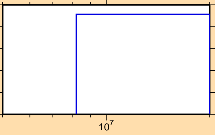
\sigma vs. E for ^{175}\text{W}(n,3n)
