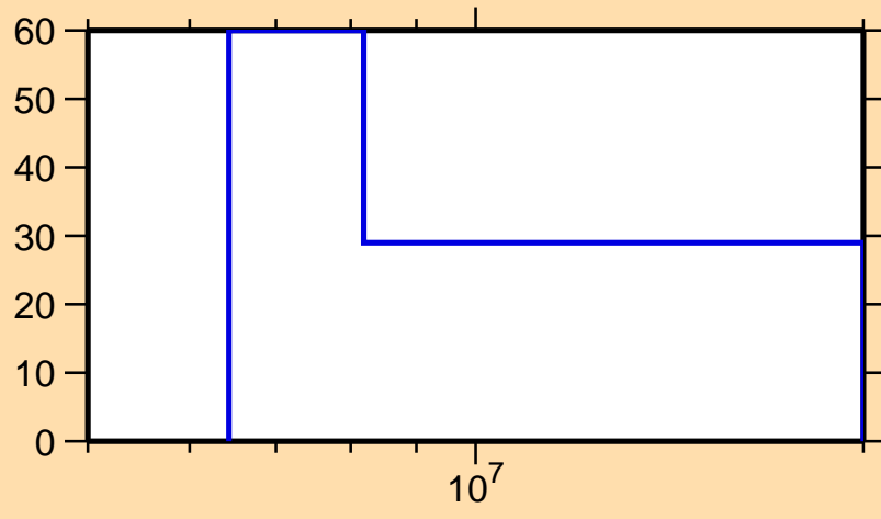
\Delta\sigma/\sigma vs. E for ^{175}\text{W}(n,2n)
