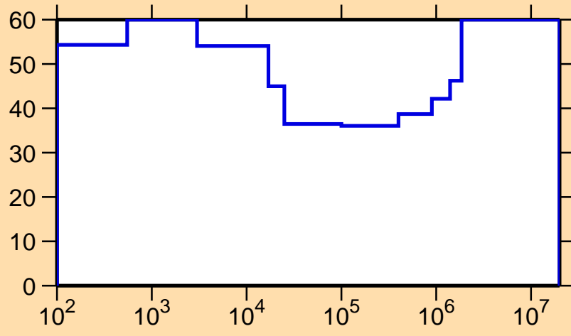
\Delta\sigma/\sigma vs. E for ^{175}\text{W}(n,\gamma)
