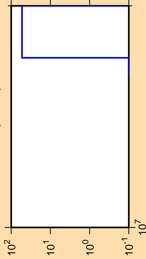
\Delta\sigma/\sigma vs. E for ^{176}\text{W}(n,3n\alpha)
