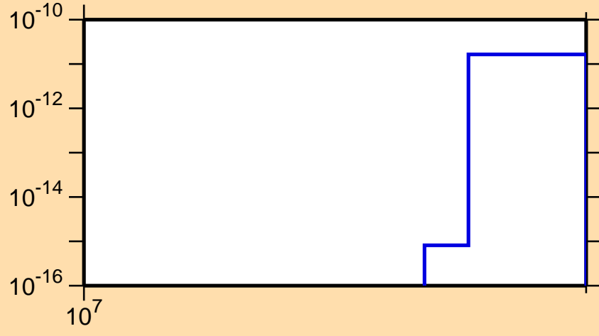
\sigma vs. E for ^{176}\text{W}(n,3n\alpha)
