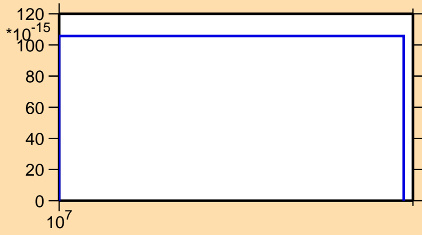
\sigma vs. E for ^{176}\text{W}(n,3n\alpha)
