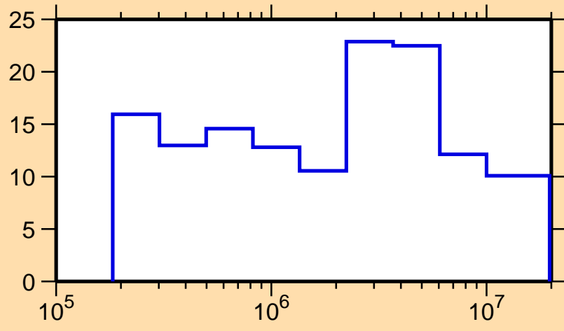
\Delta\sigma/\sigma vs. E for ^{176}\text{W}(n,el.)
