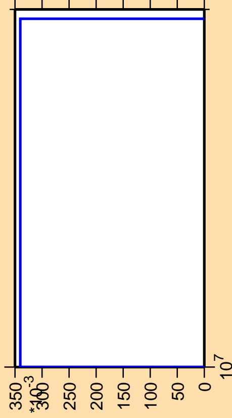
\Delta\sigma/\sigma vs. E for ^{176}\text{W}(n,3n\alpha)
