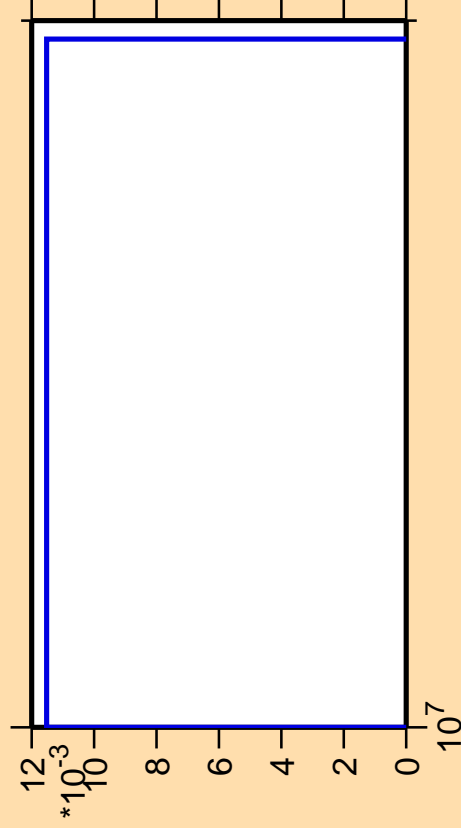
\Delta\sigma/\sigma vs. E for ^{176}\text{W} (mt 34)
