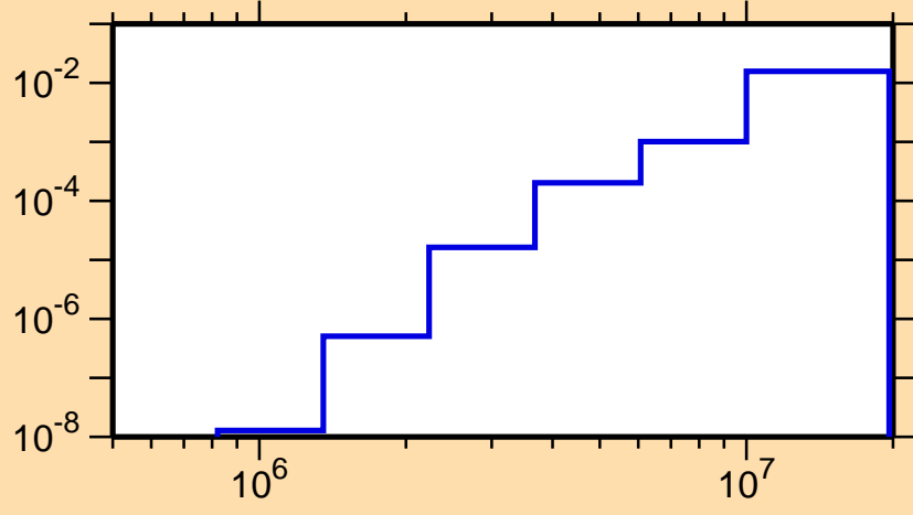
\sigma vs. E for ^{176}\text{W}(n,p)
