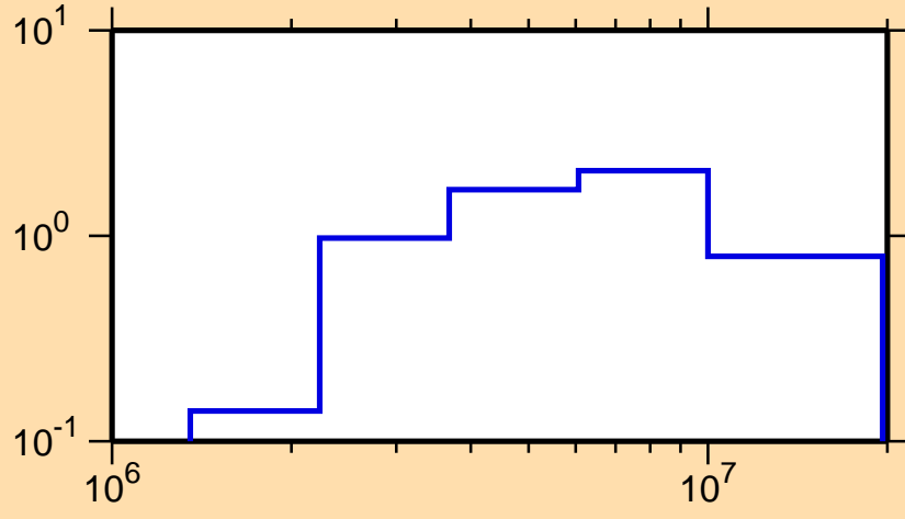
\sigma vs. E for ^{176}\text{W}(n,n\text{cont.})
