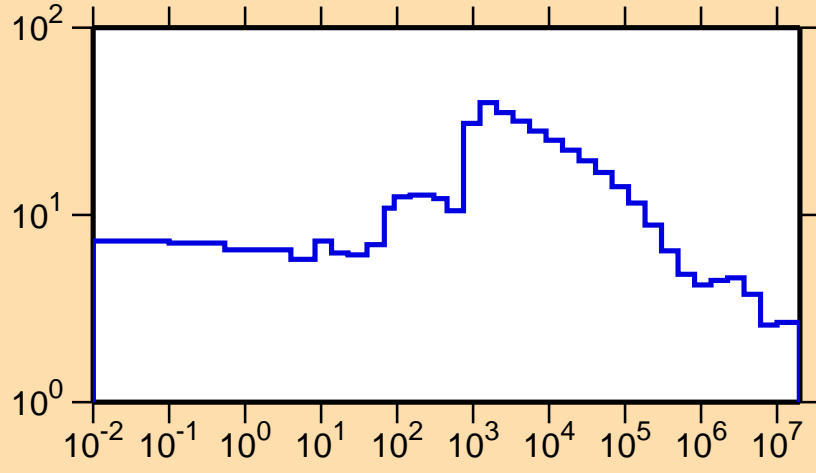
\sigma vs. E for ^{176}\text{W}(n,\text{el.})
