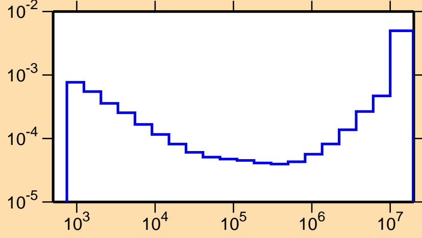
\sigma vs. E for ^{176}\text{W}(n,\alpha)
