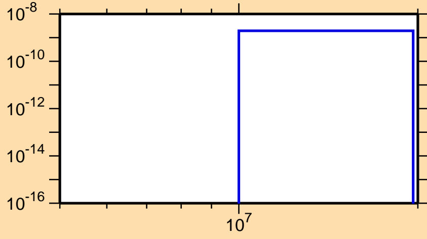
\sigma vs. E for ^{176}\text{W}(n,\text{He3})
