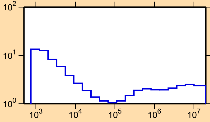
\sigma vs. E for ^{176}\text{W}(n,\text{nonel.})
