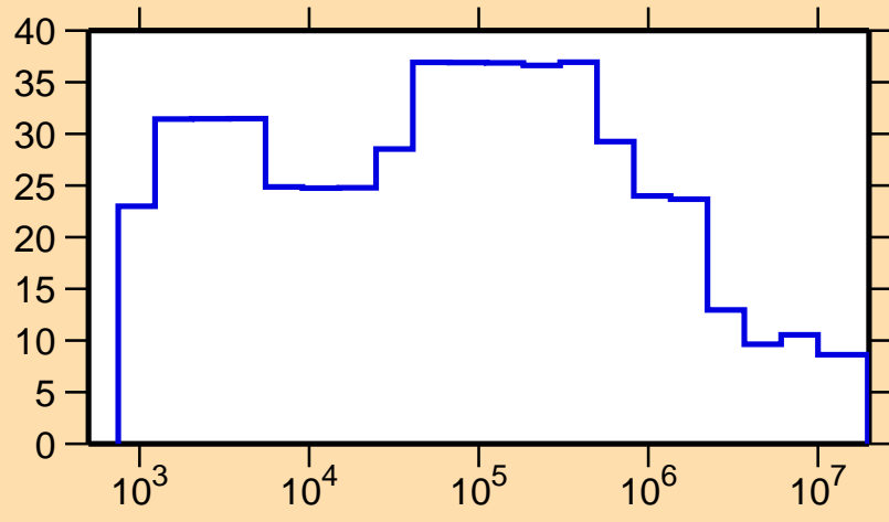
\Delta\sigma/\sigma vs. E for ^{176}\text{W}(n,\text{nonel.})
