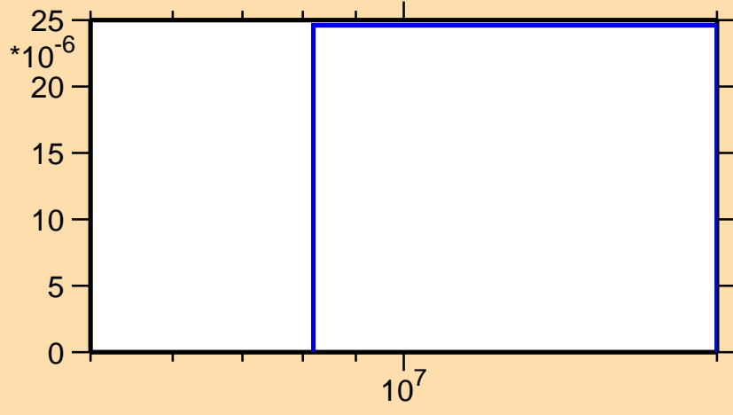
\sigma vs. E for ^{176}\text{W}(n,t)
