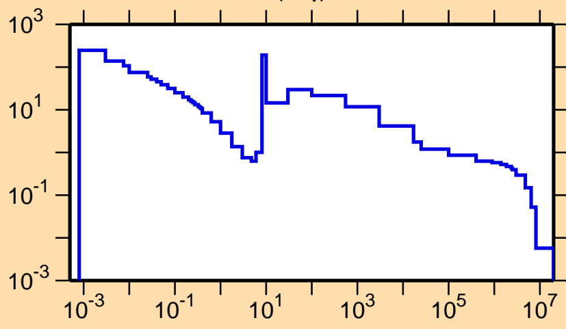
\sigma vs. E for ^{176}\text{W}(n,\gamma)
