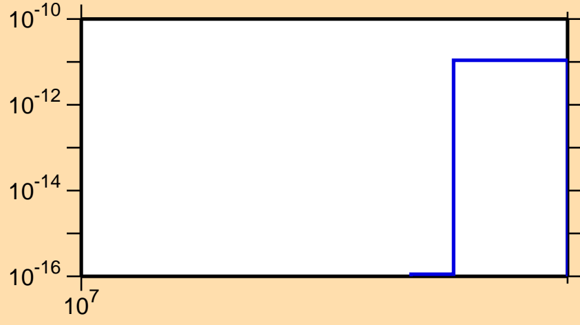
\sigma vs. E for ^{177}\text{W}(n,3n\alpha)
