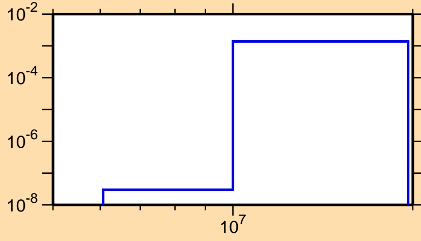
\sigma vs. E for ^{177}\text{W}(n,d)
