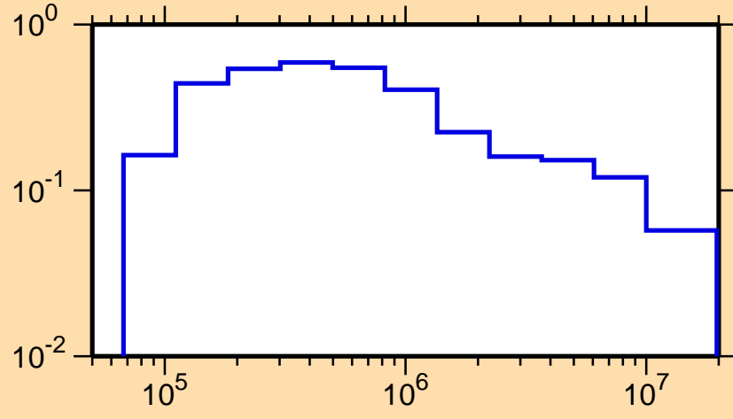
\sigma vs. E for ^{177}\text{W}(n,n_1)
